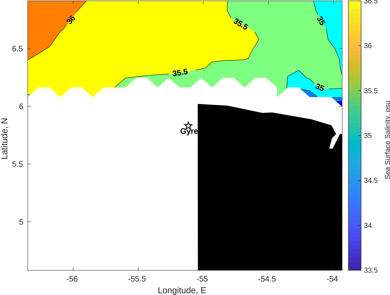
Surface Salinity for Gyre at 24-Dec-2025 00:00:00
