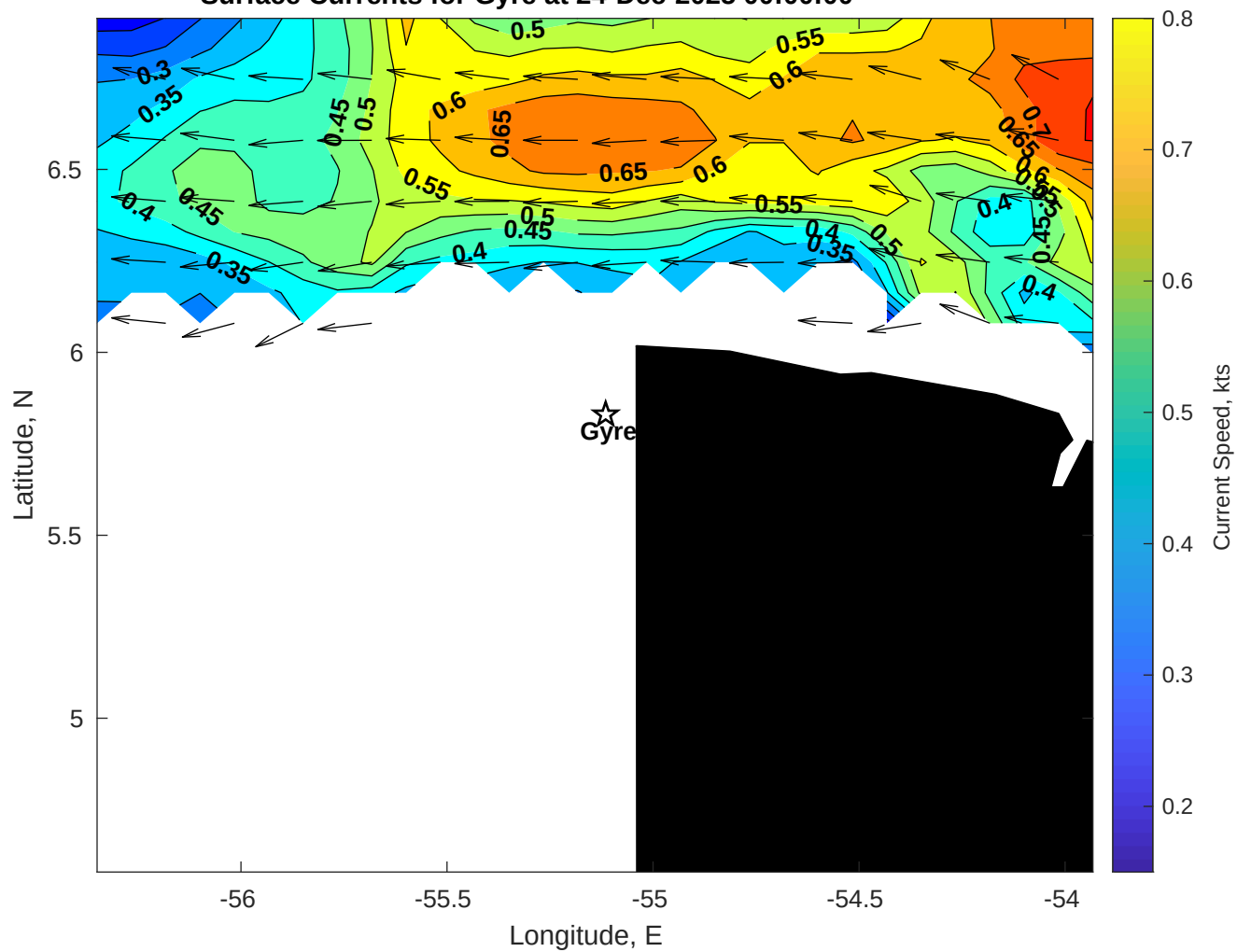
Surface Currents for Gyre at 24-Dec-2025 00:00:00
