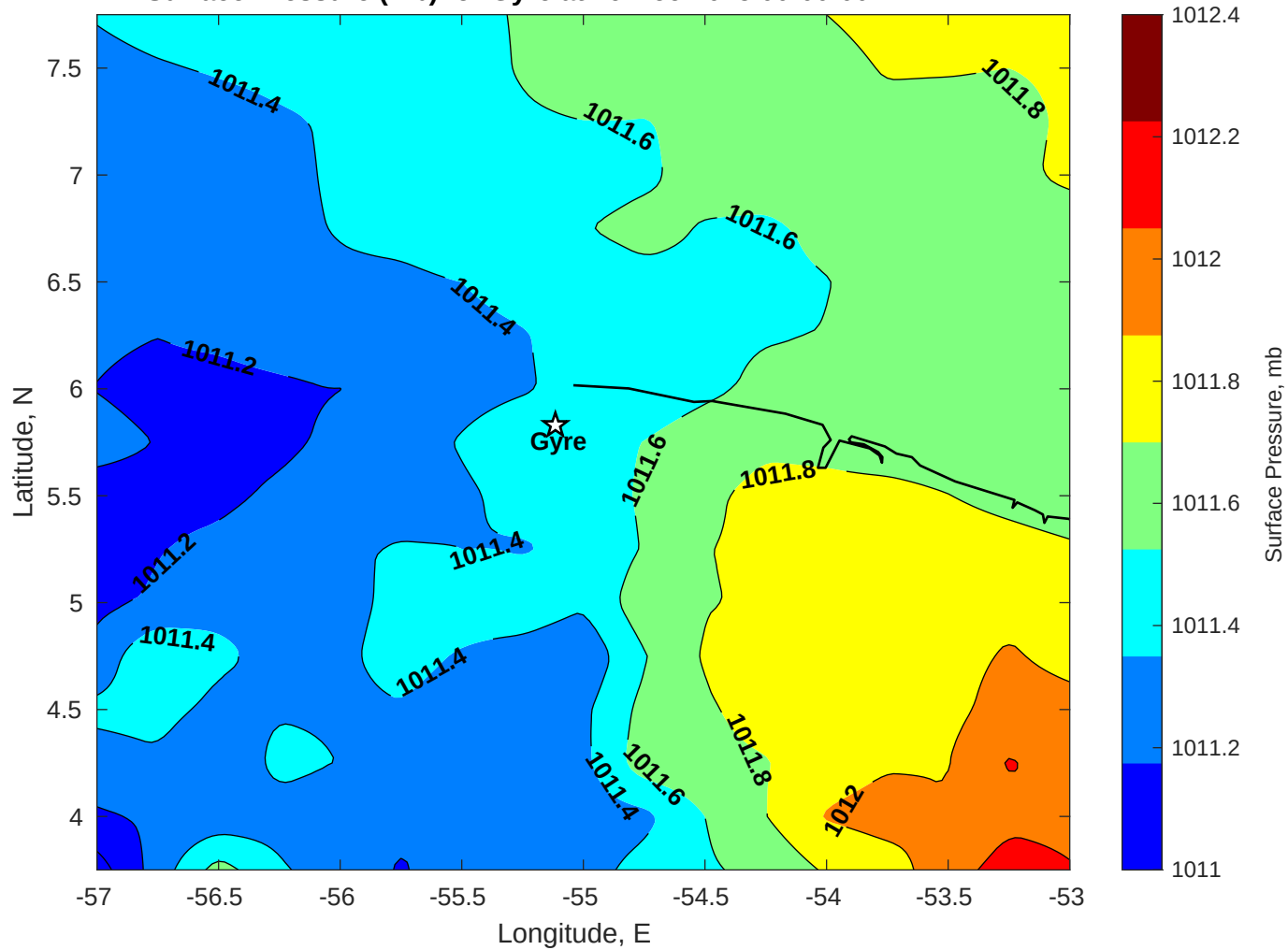
Surface Pressure (mb) for Gyre at 26-Dec-2025 00:00:00
