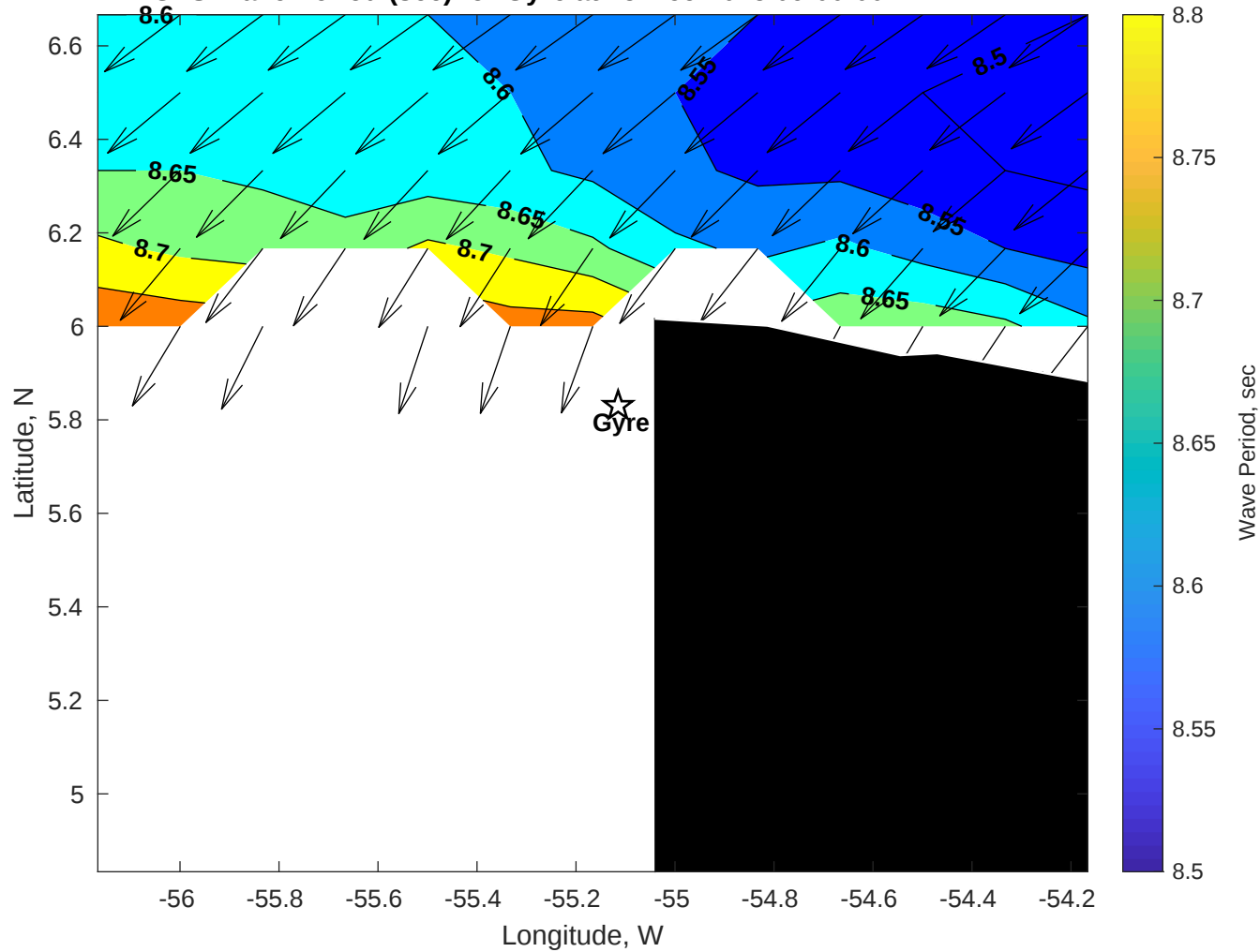
GFS Wave Period (sec) for Gyre at 25-Dec-2025 09:00:00
