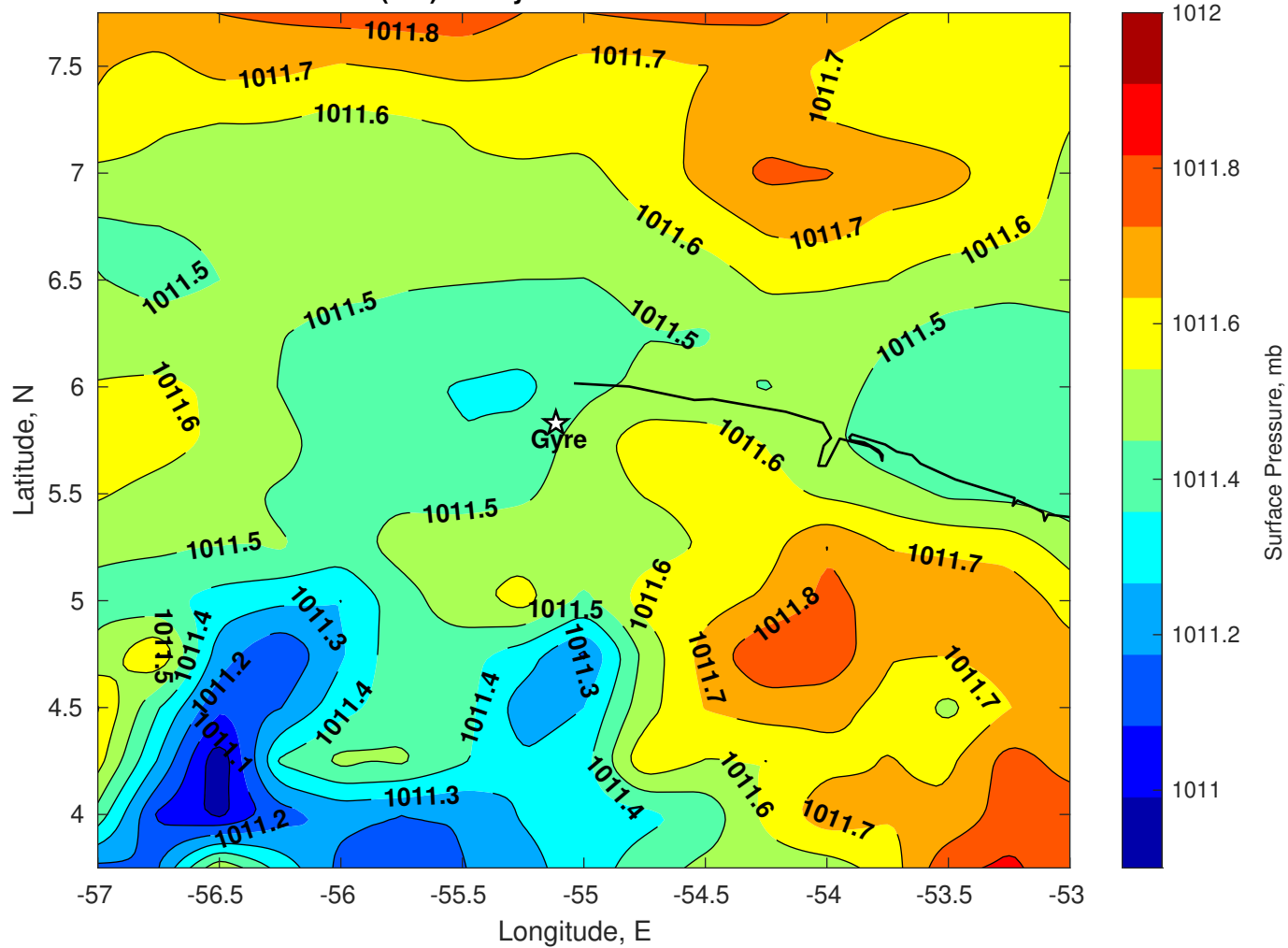
Surface Pressure (mb) for Gyre at 25-Dec-2025 00:00:00
