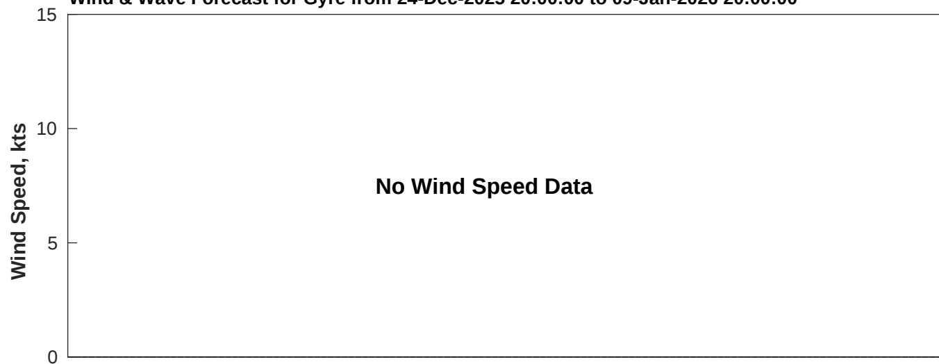
Wind & Wave Forecast for Gyre from 24-Dec-2025 20:00:00 to 09-Jan-2026 20:00:00
