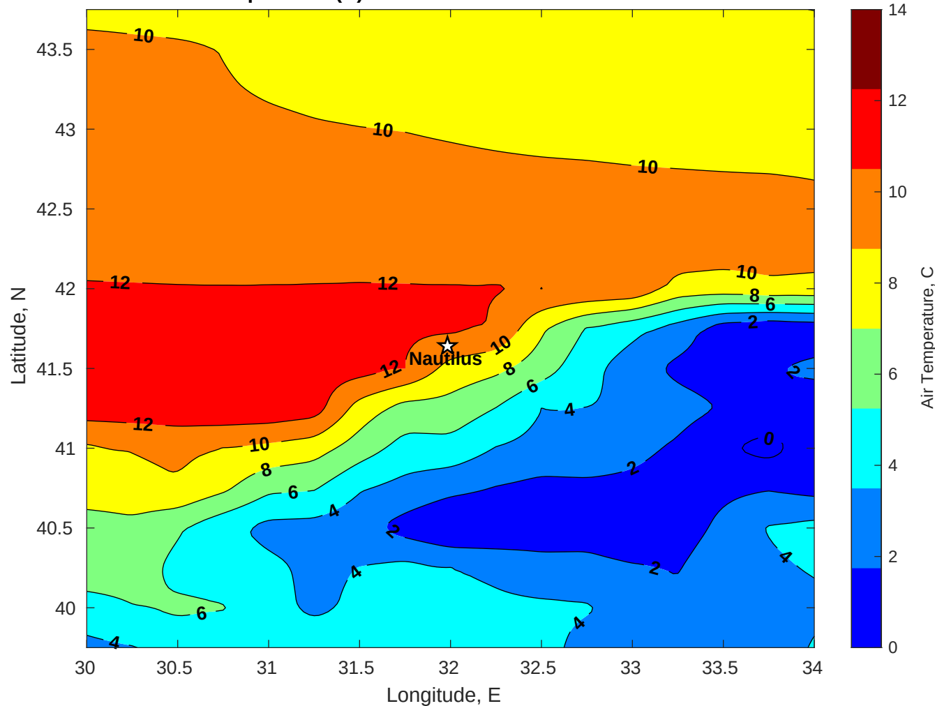
Air Temperature (C) for Nautilus at 25-Dec-2025
