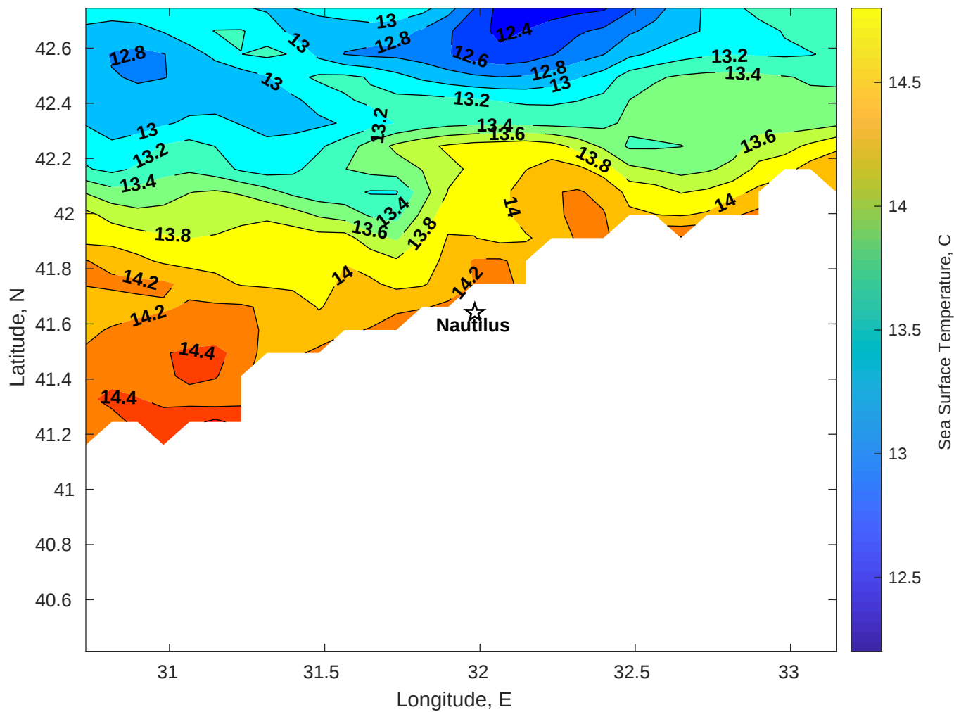
SST for Nautilus at 24-Dec-2025 00:00:00
