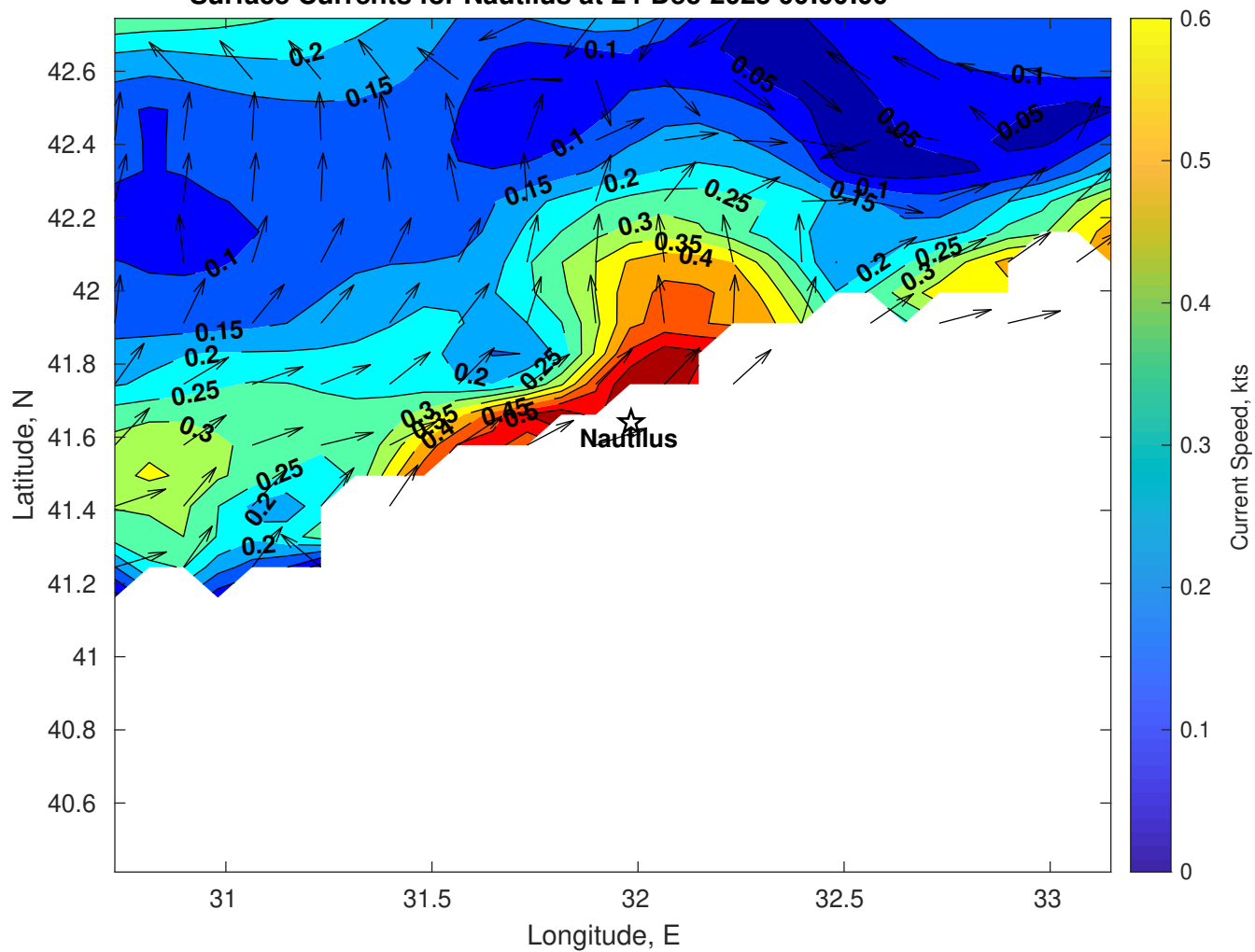
Surface Currents for Nautilus at 24-Dec-2025 00:00:00
