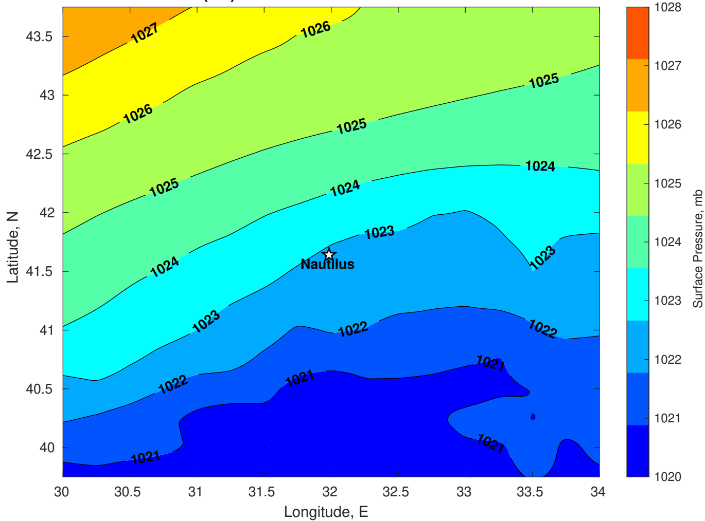
Surface Pressure (mb) for Nautilus at 26-Dec-2025 00:00:00
