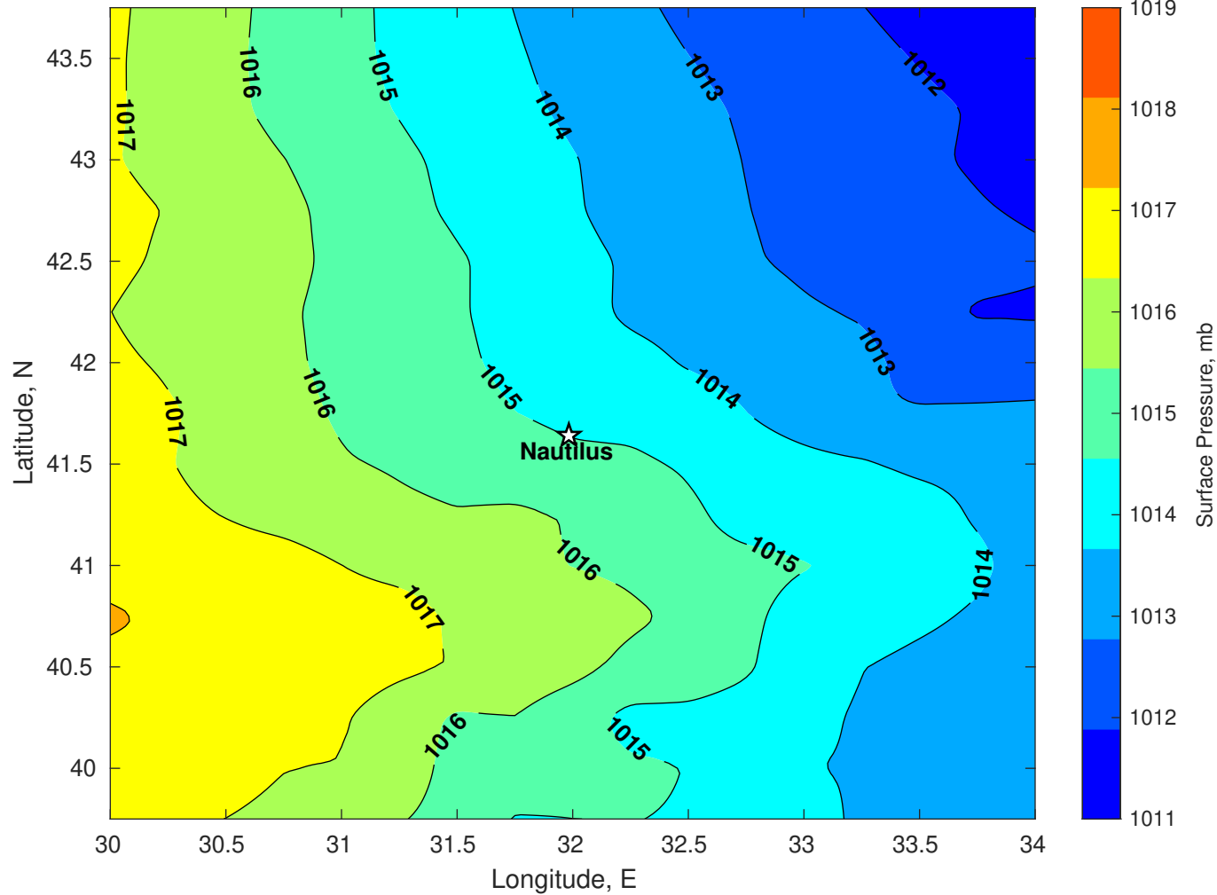
Surface Pressure (mb) for Nautilus at 27-Dec-2025 00:00:00
