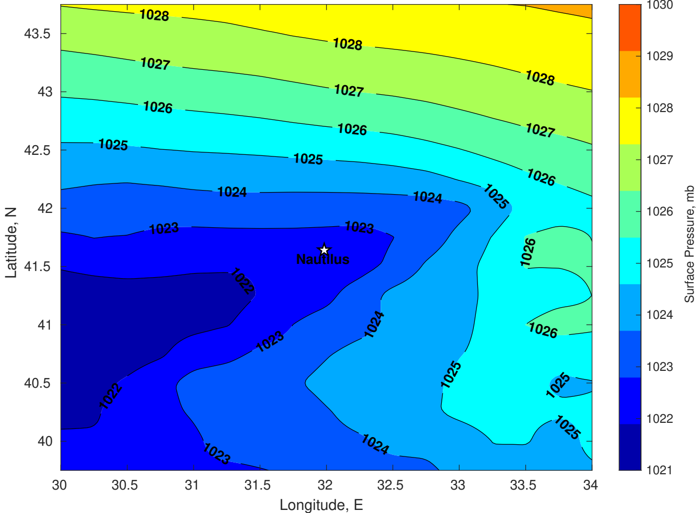
Surface Pressure (mb) for Nautilus at 25-Dec-2025 00:00:00
