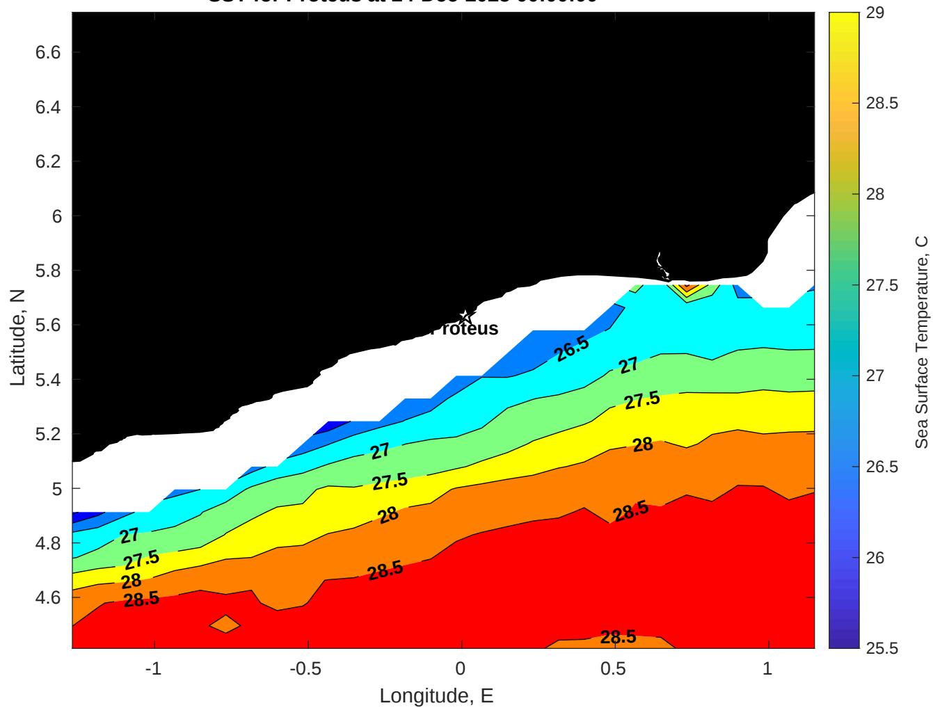
SST for Proteus at 24-Dec-2025 00:00:00
