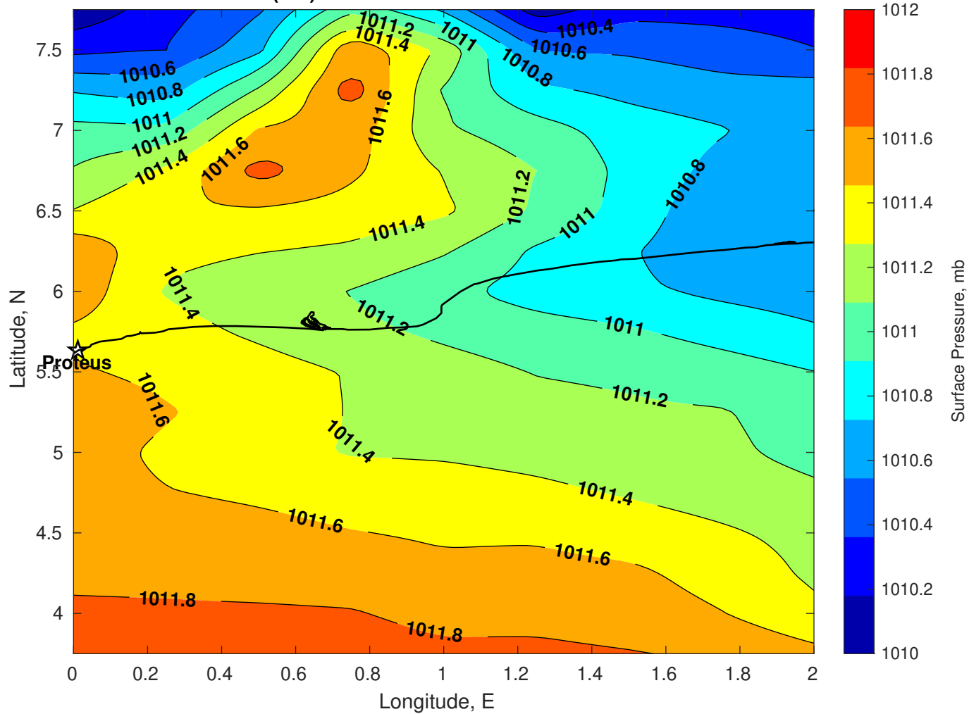
Surface Pressure (mb) for Proteus at 27-Dec-2025 00:00:00
