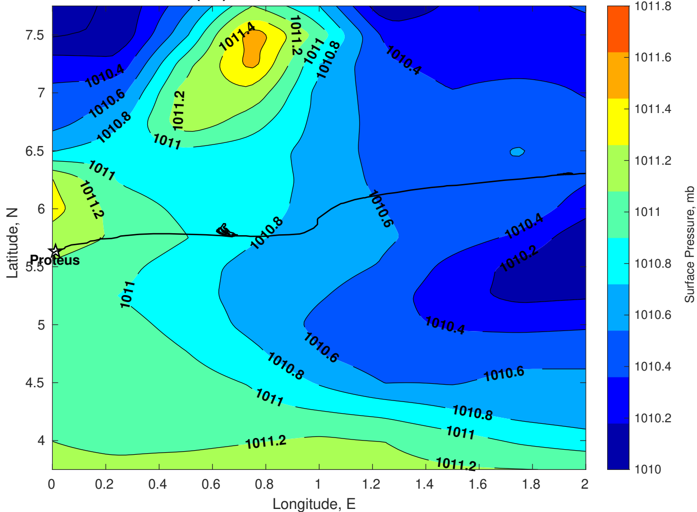
Surface Pressure (mb) for Proteus at 26-Dec-2025 00:00:00
