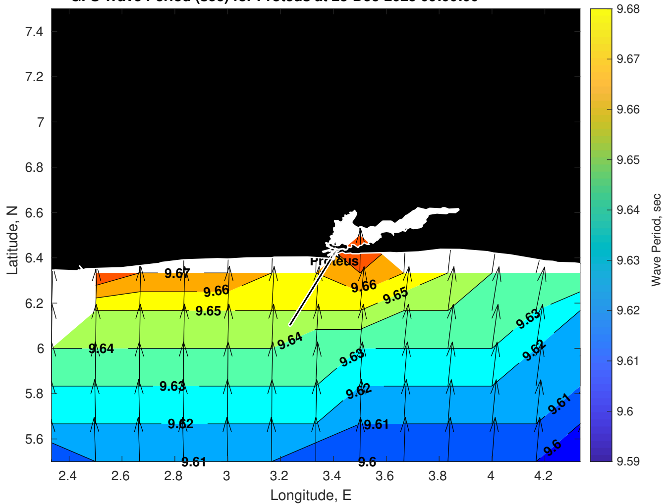
GFS Wave Period (sec) for Proteus at 23-Dec-2025 09:00:00
