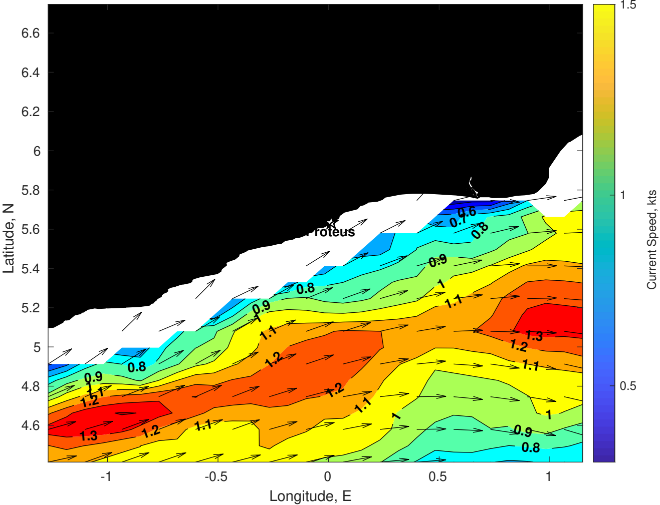
Surface Currents for Proteus at 24-Dec-2025 00:00:00
