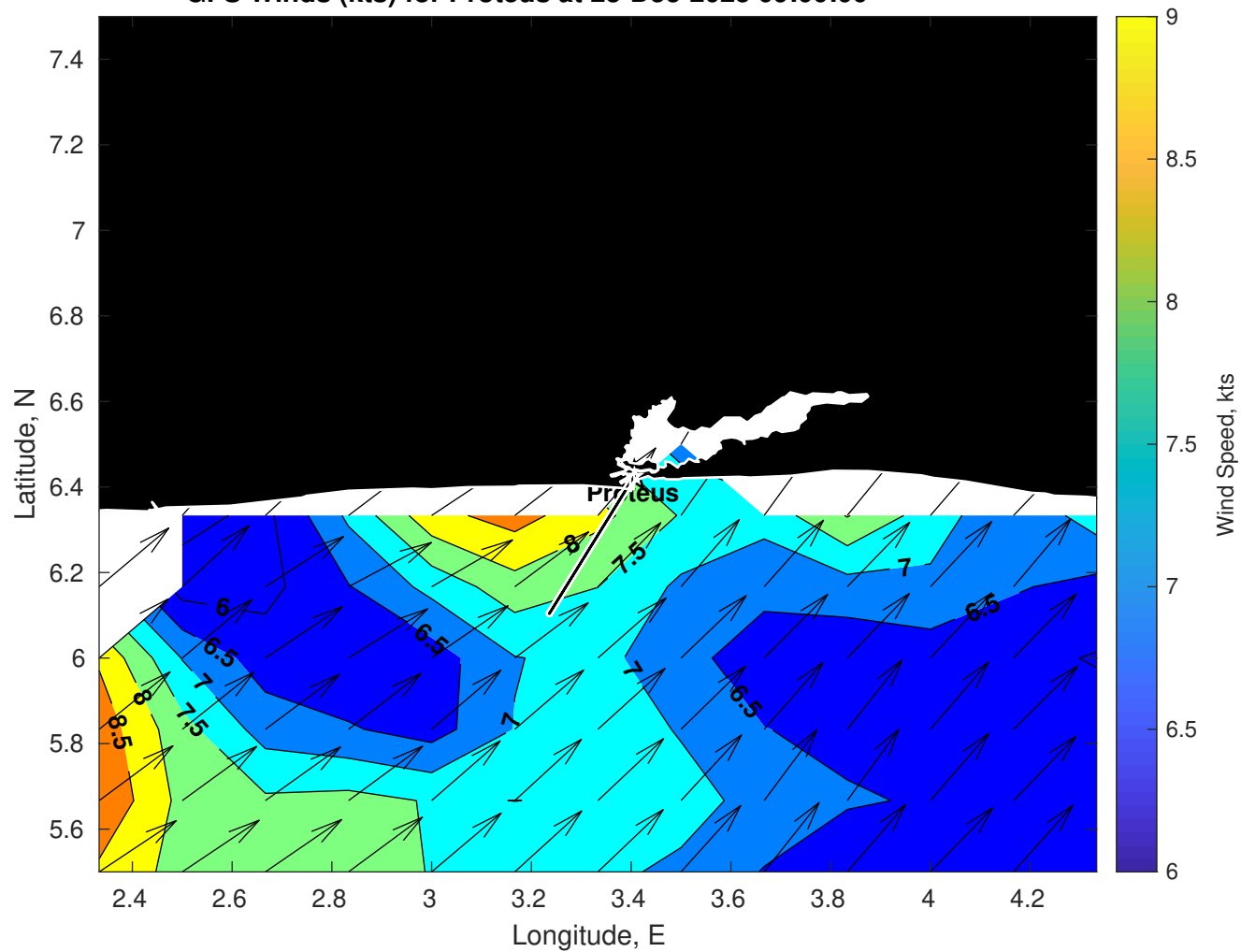
GFS Winds (kts) for Proteus at 23-Dec-2025 09:00:00
