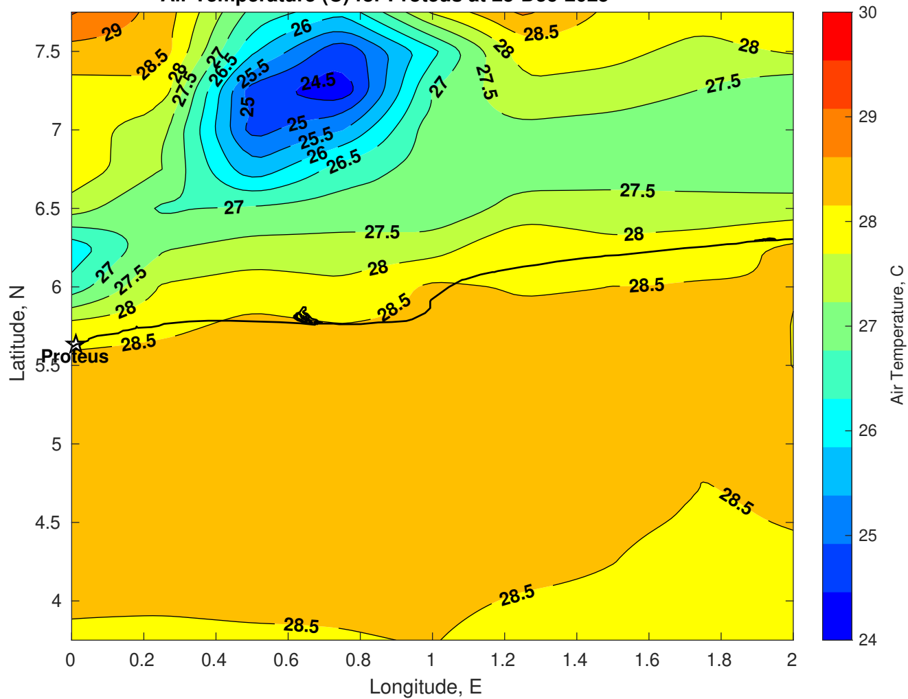
Air Temperature (C) for Proteus at 25-Dec-2025
