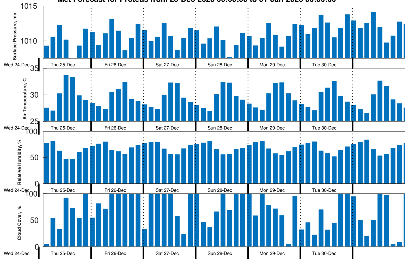
Met Forecast for Proteus from 25-Dec-2025 00:00:00 to 01-Jan-2026 00:00:00
