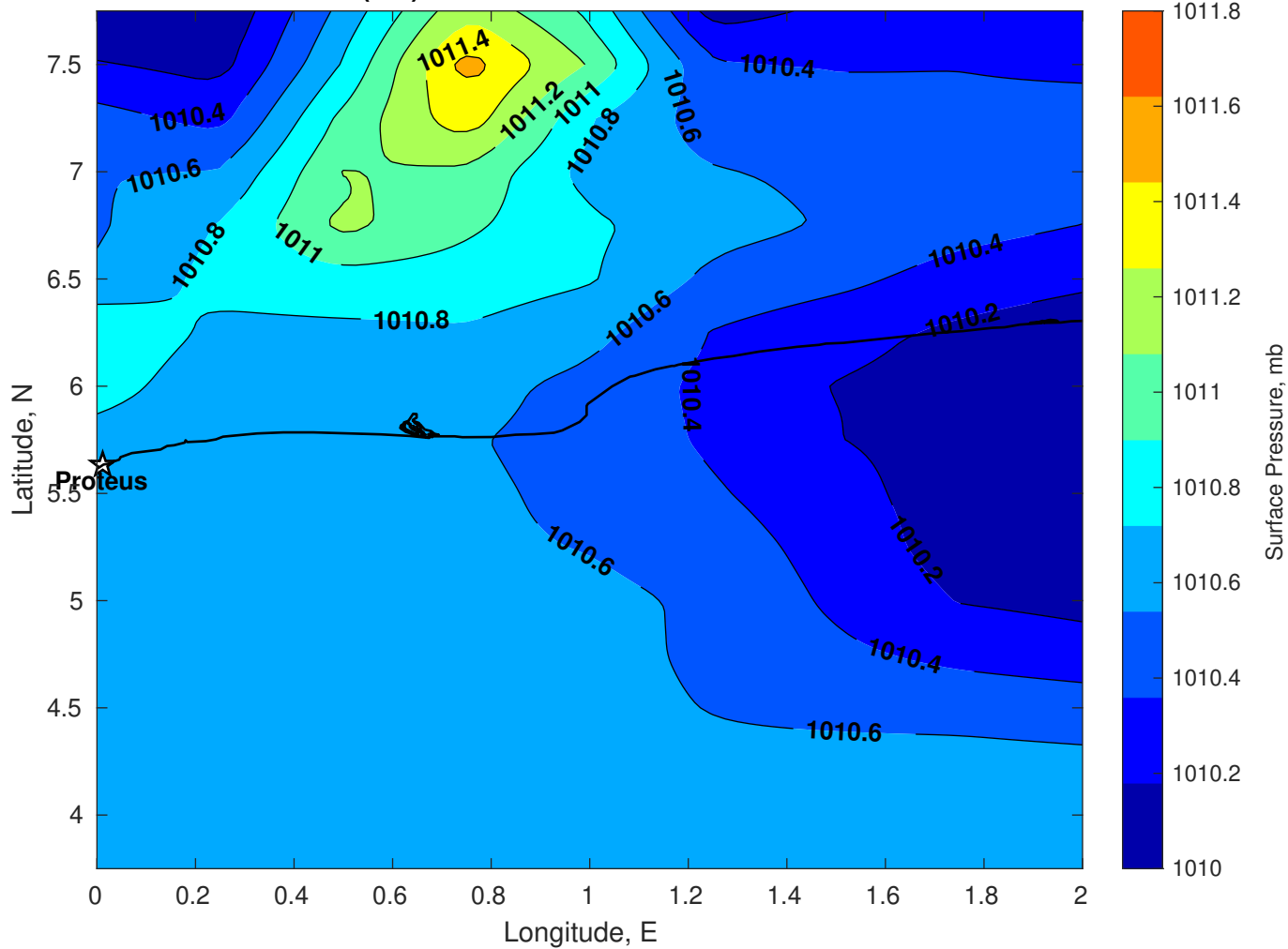
Surface Pressure (mb) for Proteus at 25-Dec-2025 00:00:00
