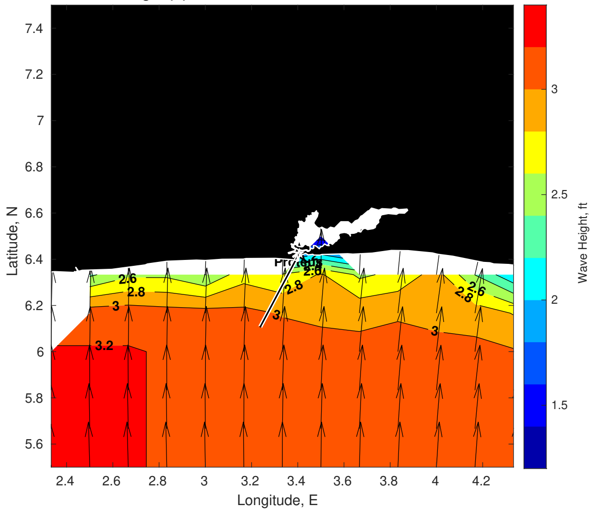
GFS Wave Height (ft) for Proteus at 23-Dec-2025 09:00:00
