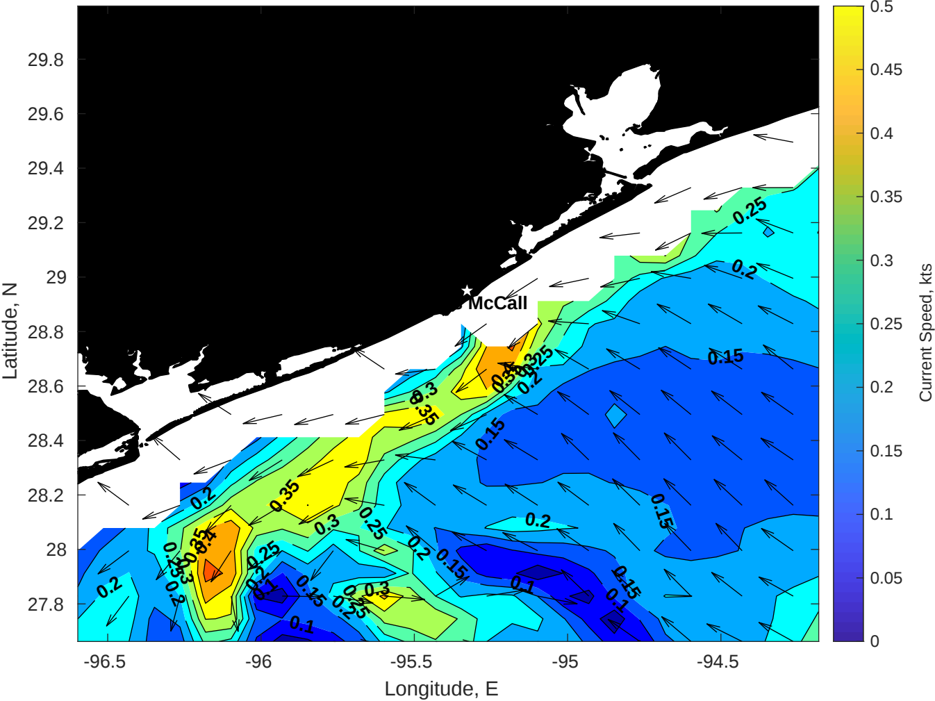
Surface Currents for Brooks McCall at 25-Dec-2025 00:00:00
