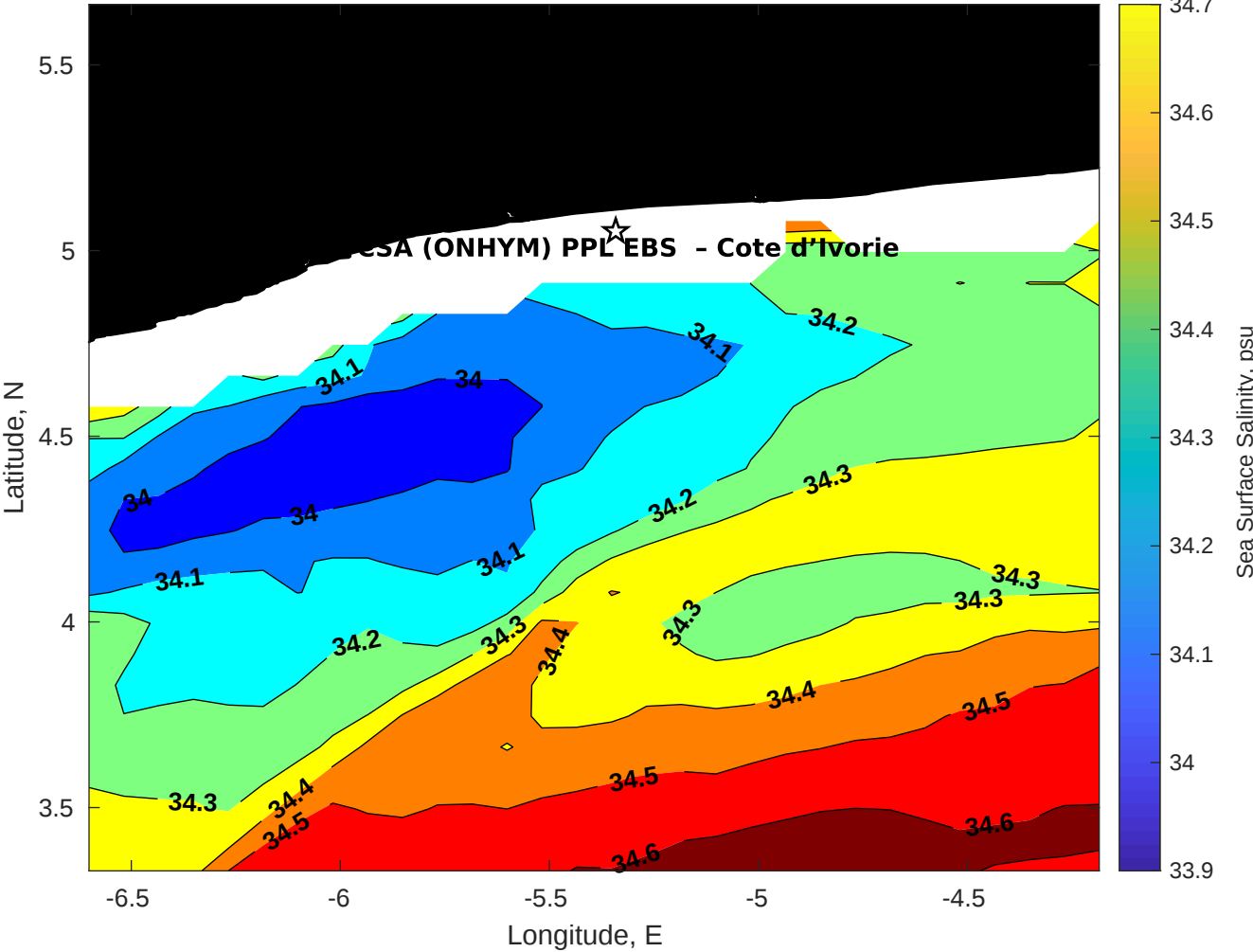
Surface Salinity for CSA (ONHYM) PPL EBS - Cote d'Ivoire at 25-Dec-2025 00:00:00
