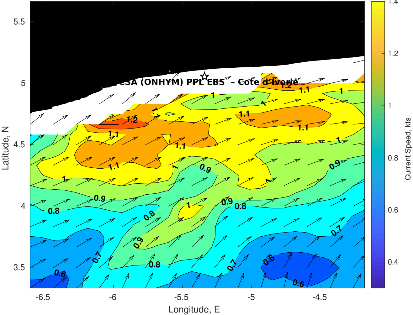
Surface Currents for CSA (ONHYM) PPL EBS - Cote d'Ivoire at 25-Dec-2025 00:00:00
