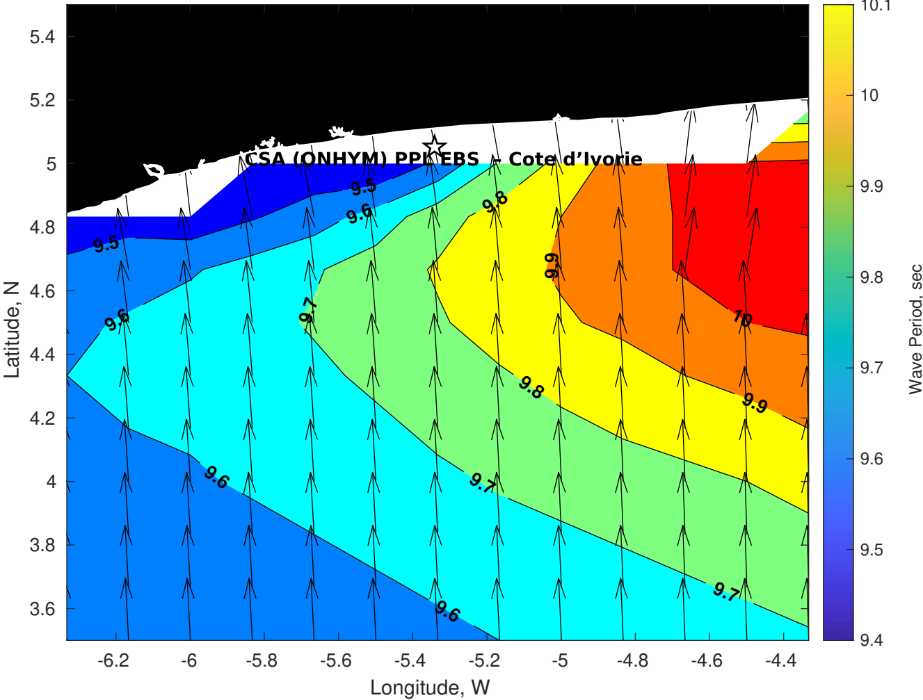
GFS Wave Period (sec) for CSA (ONHYM) PPL EBS - Cote d'Ivoire at 26-Dec-2025 09:00:00
