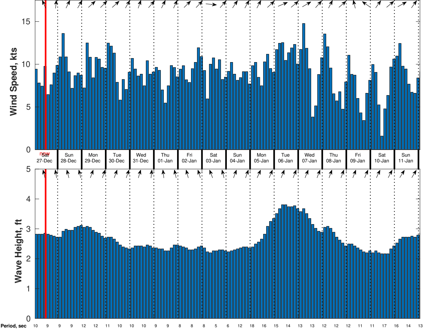
Wind & Wave Forecast for CSA (ONHYM) PPL EBS - Cote d'Ivoire from 26-Dec-2025 01:00:00 to 11-Jan-2026 01:00:00
