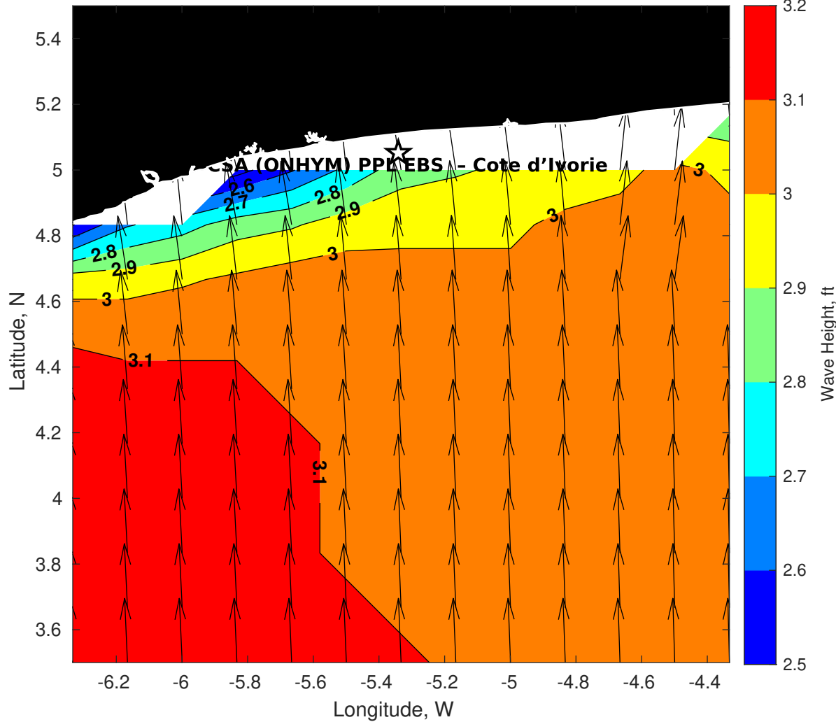
GFS Wave Height (ft) for CSA (ONHYM) PPL EBS - Cote d'Ivoire at 26-Dec-2025 09:00:00
