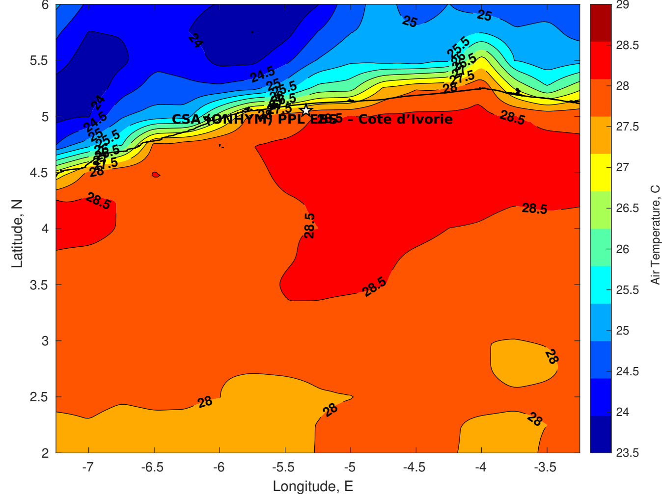
Air Temperature (C) for CSA (ONHYM) PPL EBS - Cote d'Ivoire at 26-Dec-2025
