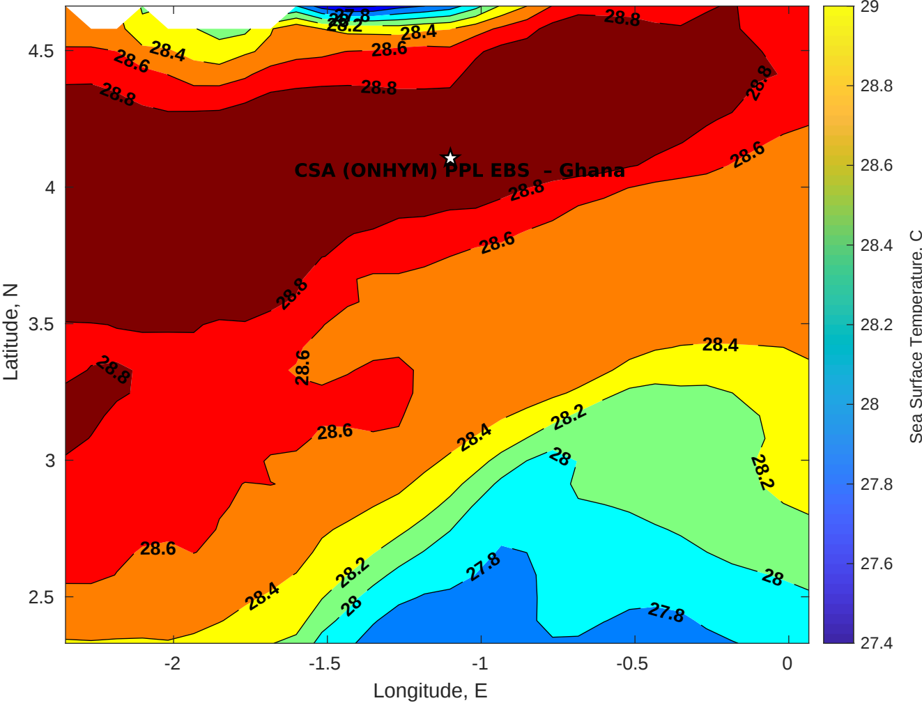
SST for CSA (ONHYM) PPL EBS - Ghana at 25-Dec-2025 00:00:00
