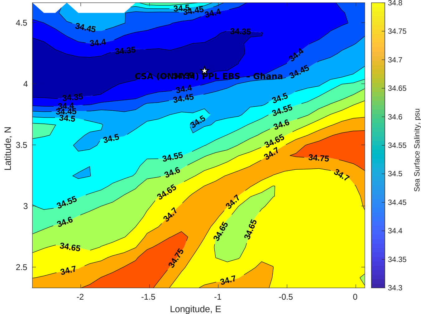
Surface Salinity for CSA (ONHYM) PPL EBS - Ghana at 25-Dec-2025 00:00:00
