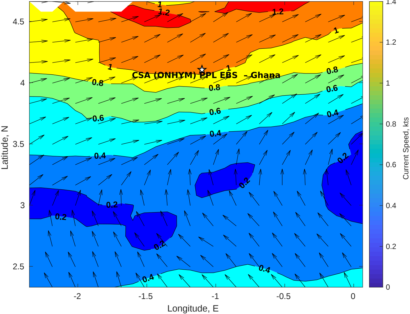
Surface Currents for CSA (ONHYM) PPL EBS - Ghana at 25-Dec-2025 00:00:00
