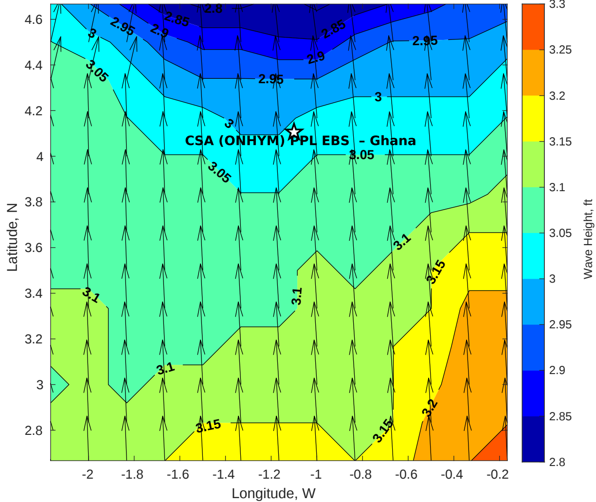
GFS Wave Height (ft) for CSA (ONHYM) PPL EBS - Ghana at 26-Dec-2025 09:00:00
