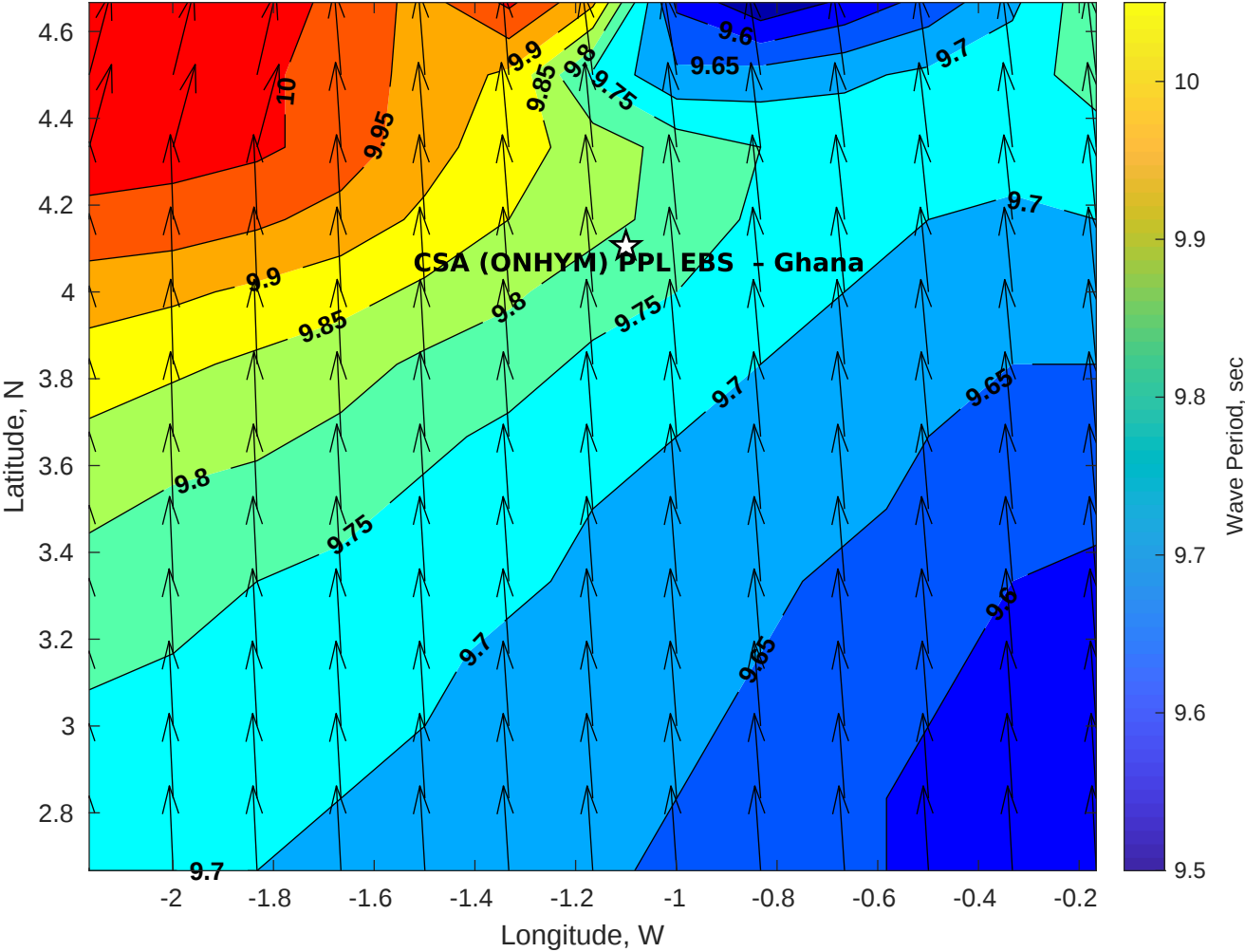
GFS Wave Period (sec) for CSA (ONHYM) PPL EBS - Ghana at 26-Dec-2025 09:00:00
