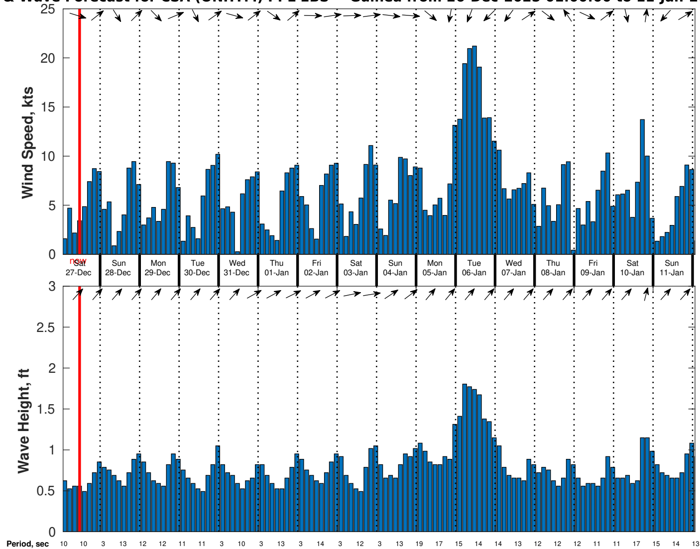
Wind & Wave Forecast for CSA (ONHYM) PPL EBS - Guinea from 26-Dec-2025 01:00:00 to 11-Jan-2026 01:00:00
