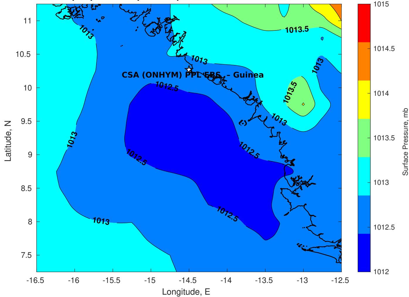
Surface Pressure (mb) for CSA (ONHYM) PPL EBS - Guinea at 27-Dec-2025 00:00:00
