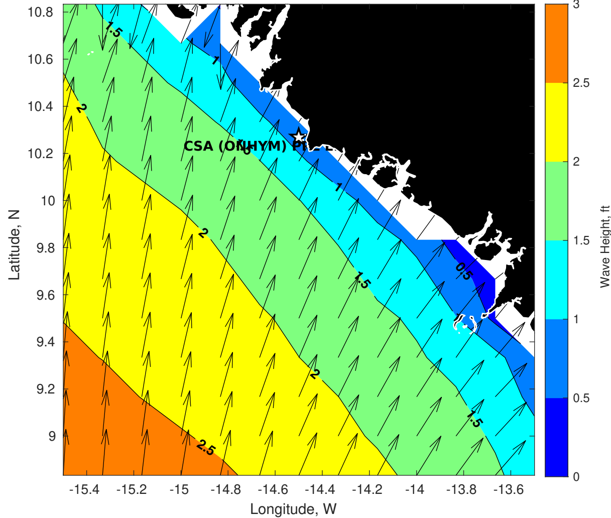
GFS Wave Height (ft) for CSA (ONHYM) PPL EBS - Guinea at 26-Dec-2025 09:00:00
