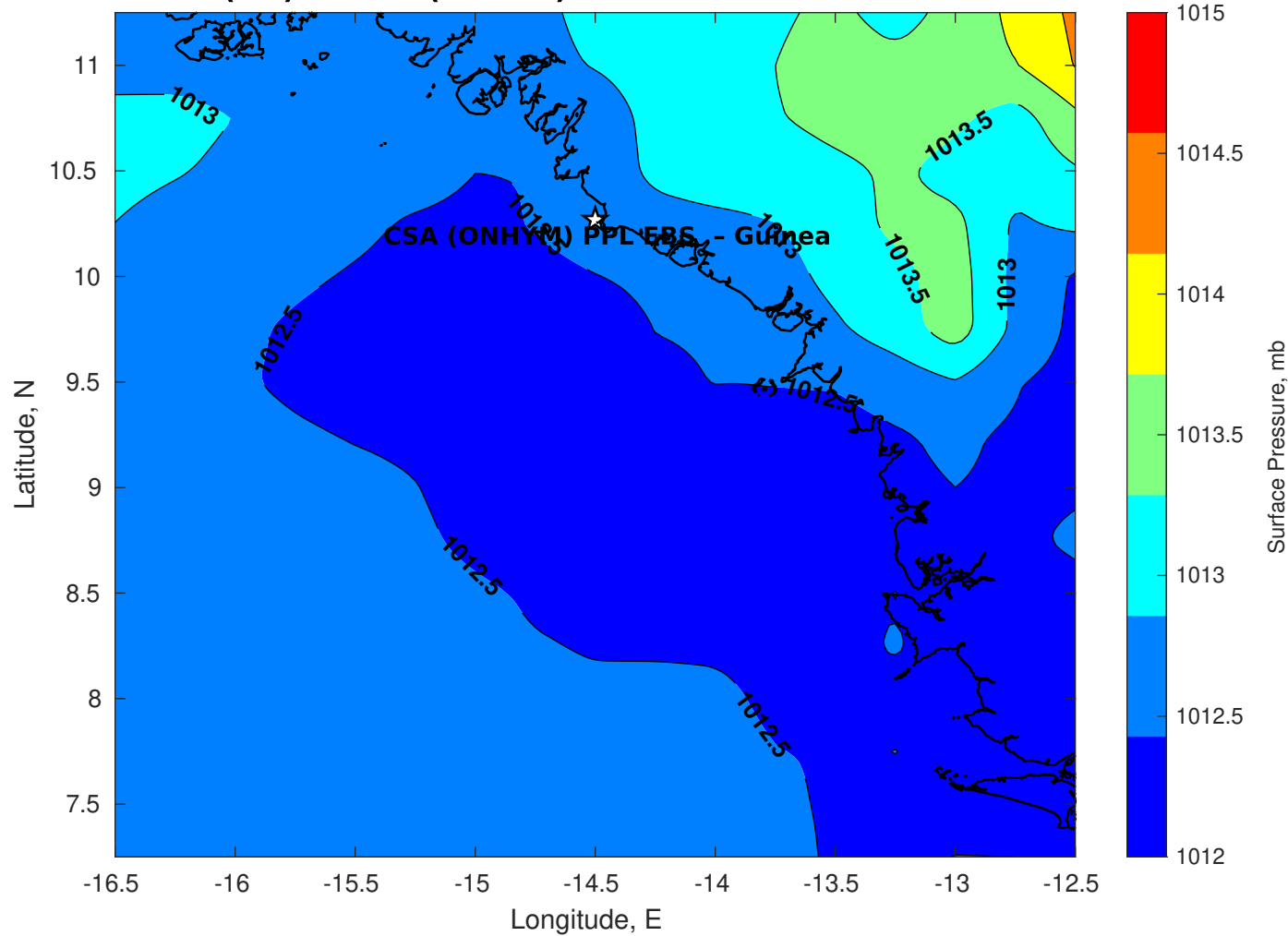
Surface Pressure (mb) for CSA (ONHYM) PPL EBS - Guinea at 28-Dec-2025 00:00:00
