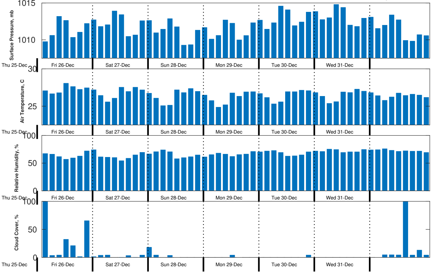
Met Forecast for CSA (ONHYM) PPL EBS - Guinea from 26-Dec-2025 00:00:00 to 02-Jan-2026 00:00:00
