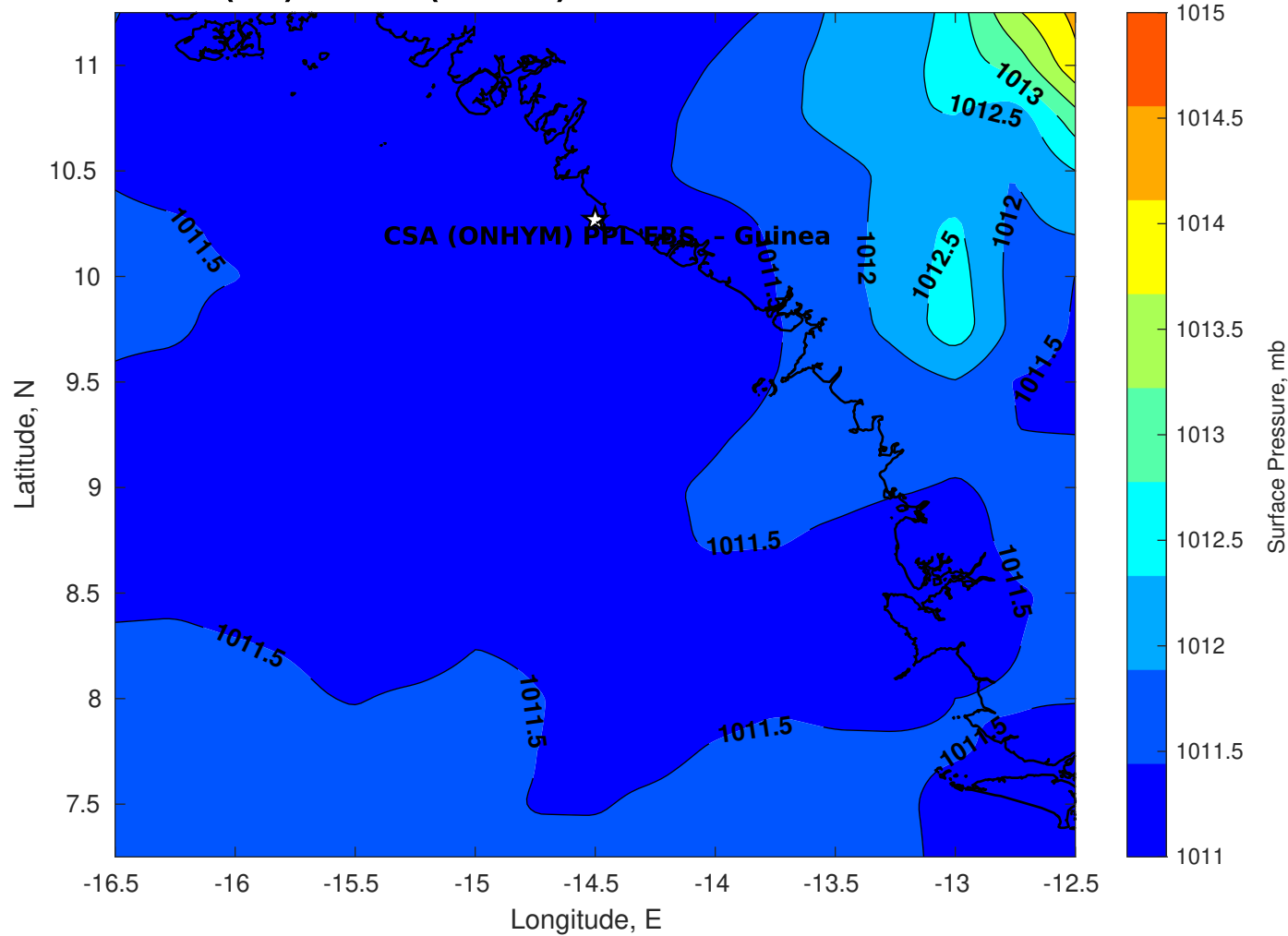
Surface Pressure (mb) for CSA (ONHYM) PPL EBS - Guinea at 26-Dec-2025 00:00:00
