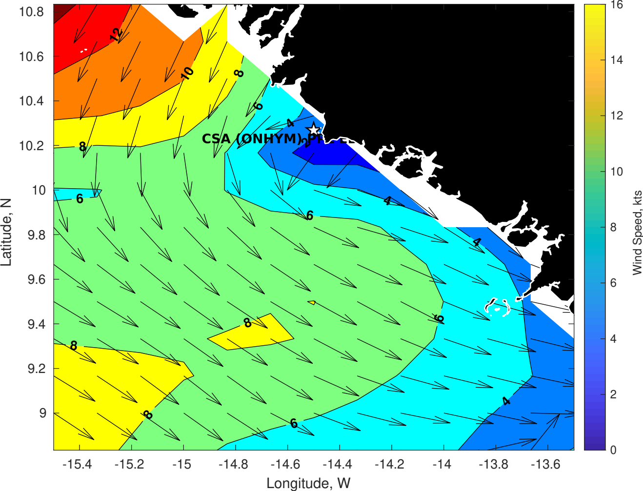
GFS Winds (kts) for CSA (ONHYM) PPL EBS - Guinea at 26-Dec-2025 09:00:00
