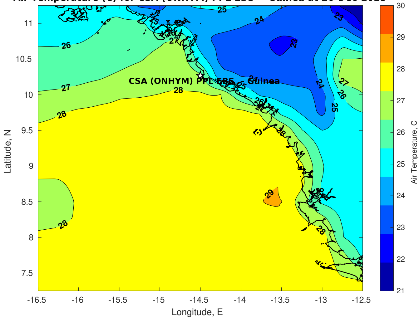
Air Temperature (C) for CSA (ONHYM) PPL EBS - Guinea at 26-Dec-2025
