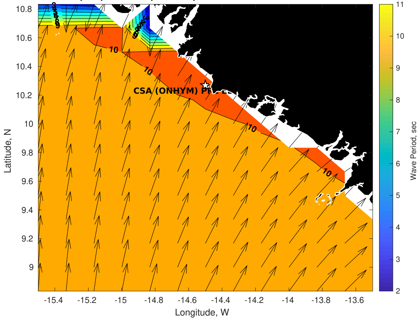
GFS Wave Period (sec) for CSA (ONHYM) PPL EBS - Guinea at 26-Dec-2025 09:00:00
