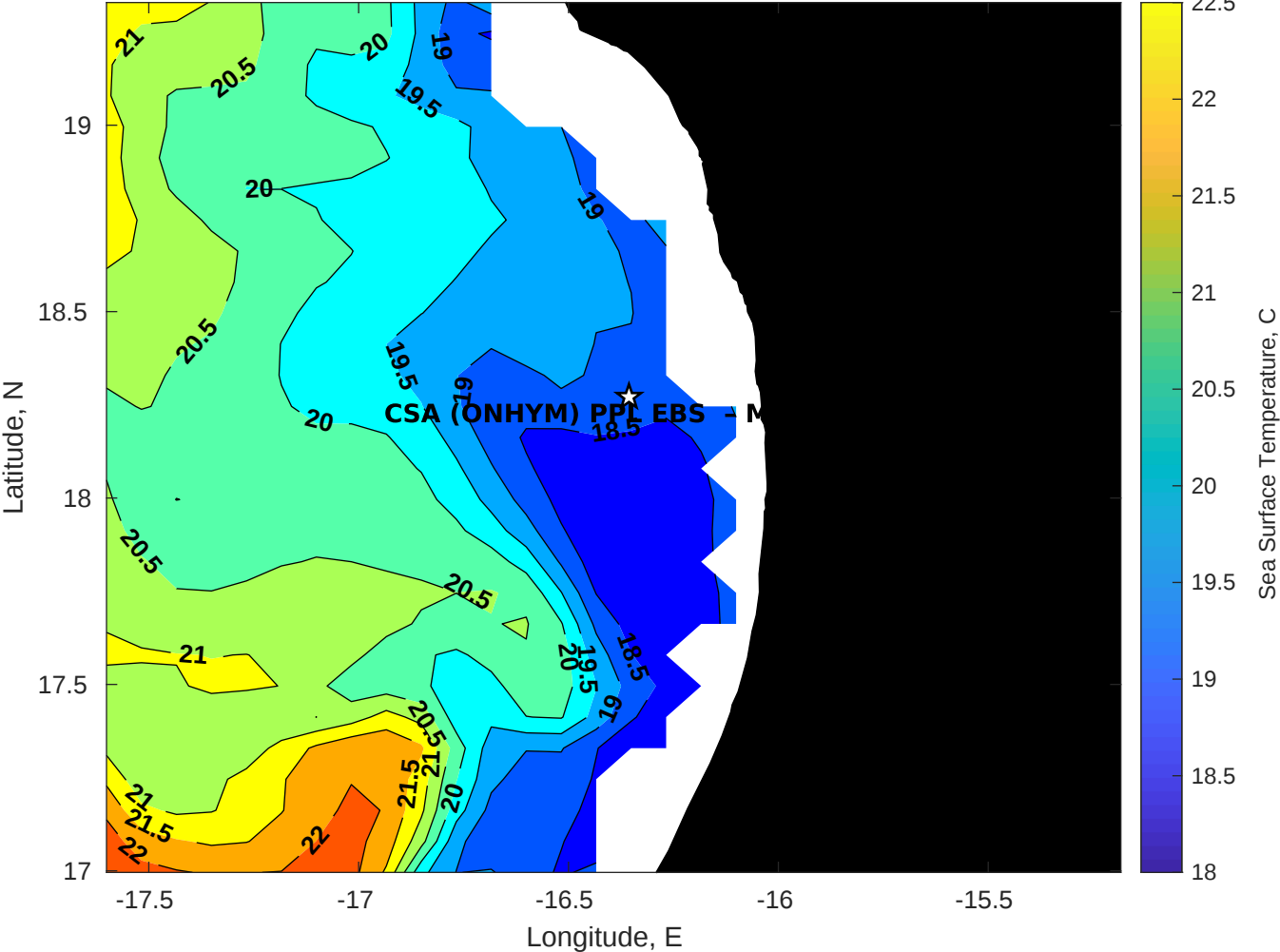
SST for CSA (ONHYM) PPL EBS - Mauritania at 25-Dec-2025 00:00:00
