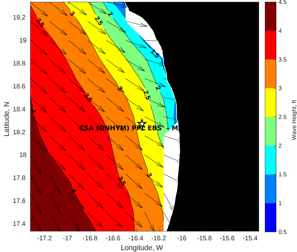
GFS Wave Height (ft) for CSA (ONHYM) PPL EBS - Mauritania at 26-Dec-2025 09:00:00
