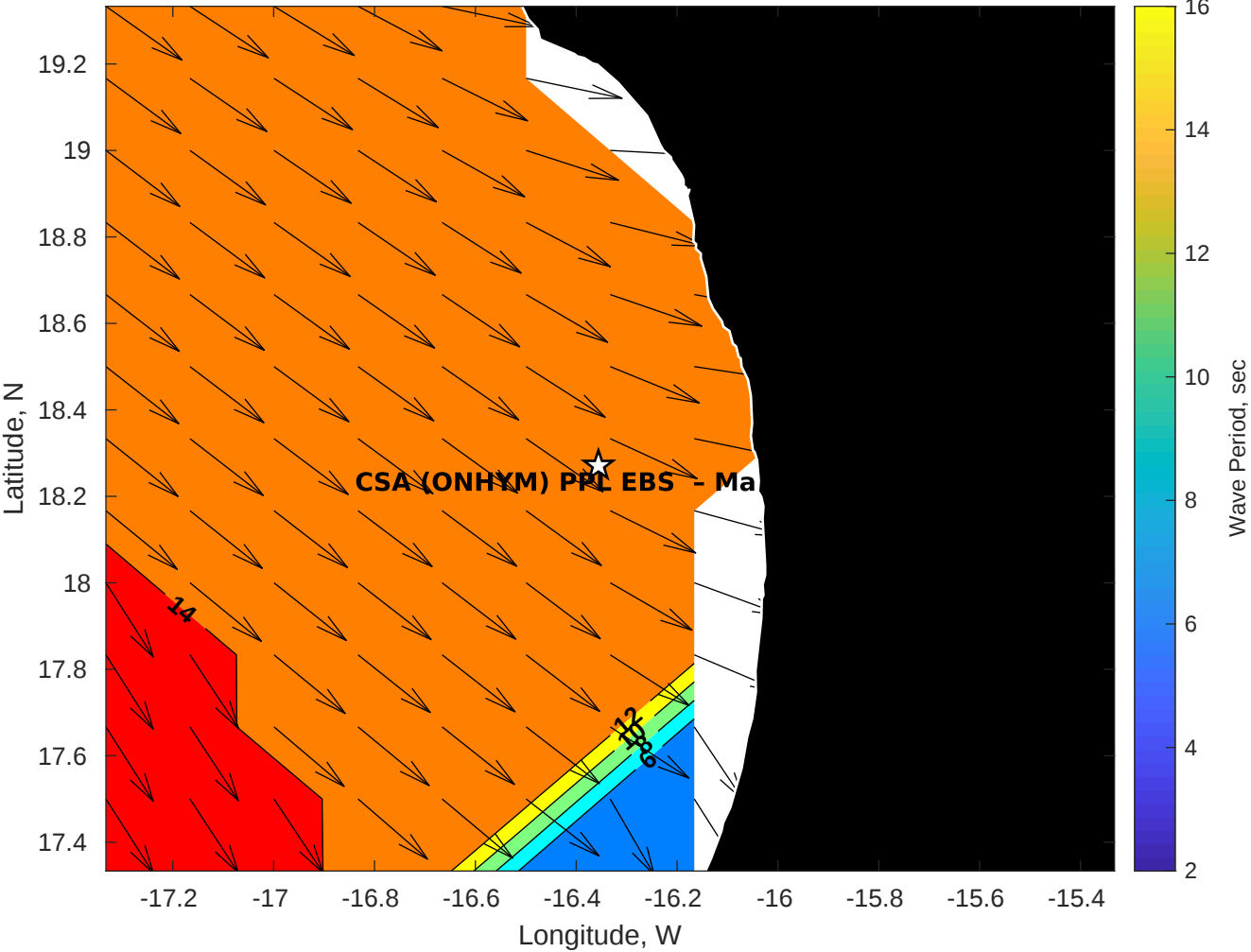
GFS Wave Period (sec) for CSA (ONHYM) PPL EBS - Mauritania at 26-Dec-2025 09:00:00
