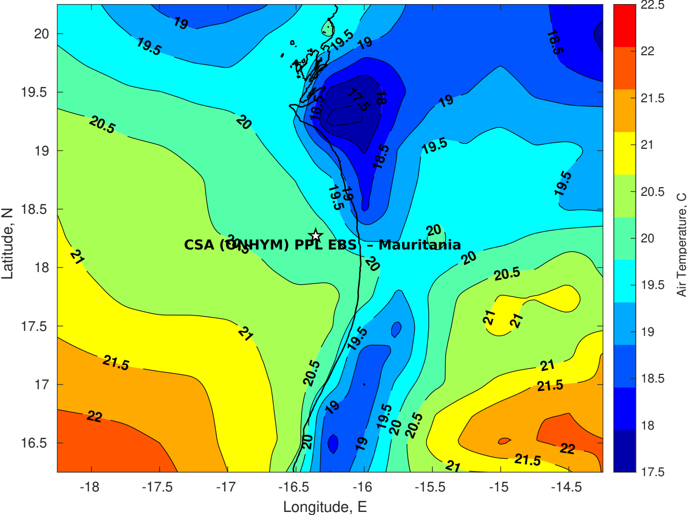
Air Temperature (C) for CSA (ONHYM) PPL EBS - Mauritania at 26-Dec-2025
