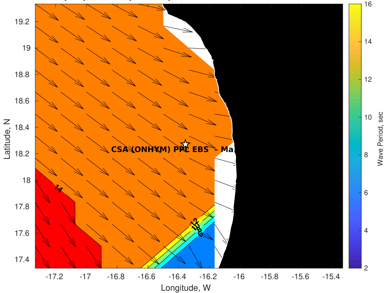
GFS Wave Period (sec) for CSA (ONHYM) PPL EBS - Mauritania at 26-Dec-2025 09:00:00
