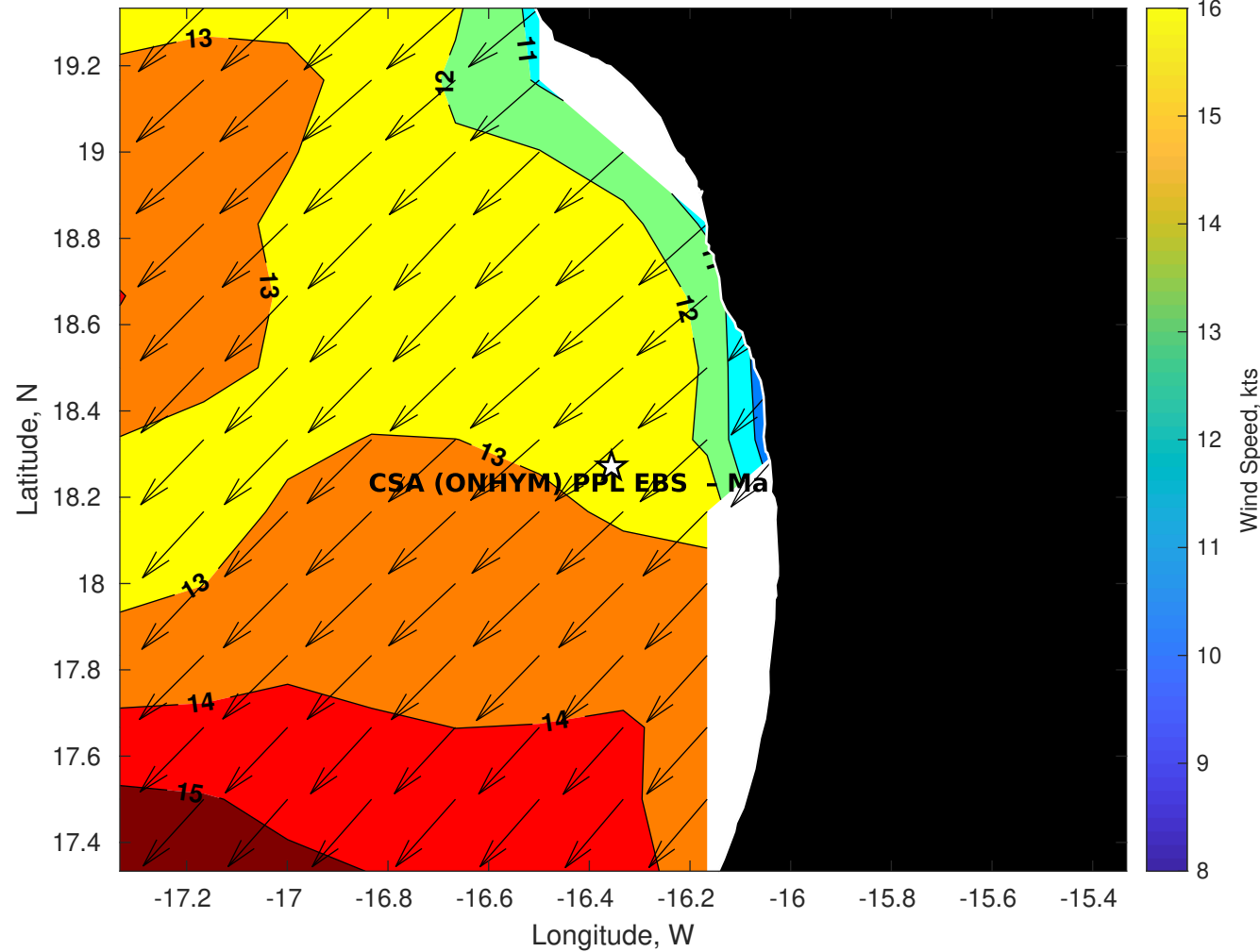
GFS Winds (kts) for CSA (ONHYM) PPL EBS - Mauritania at 26-Dec-2025 09:00:00
