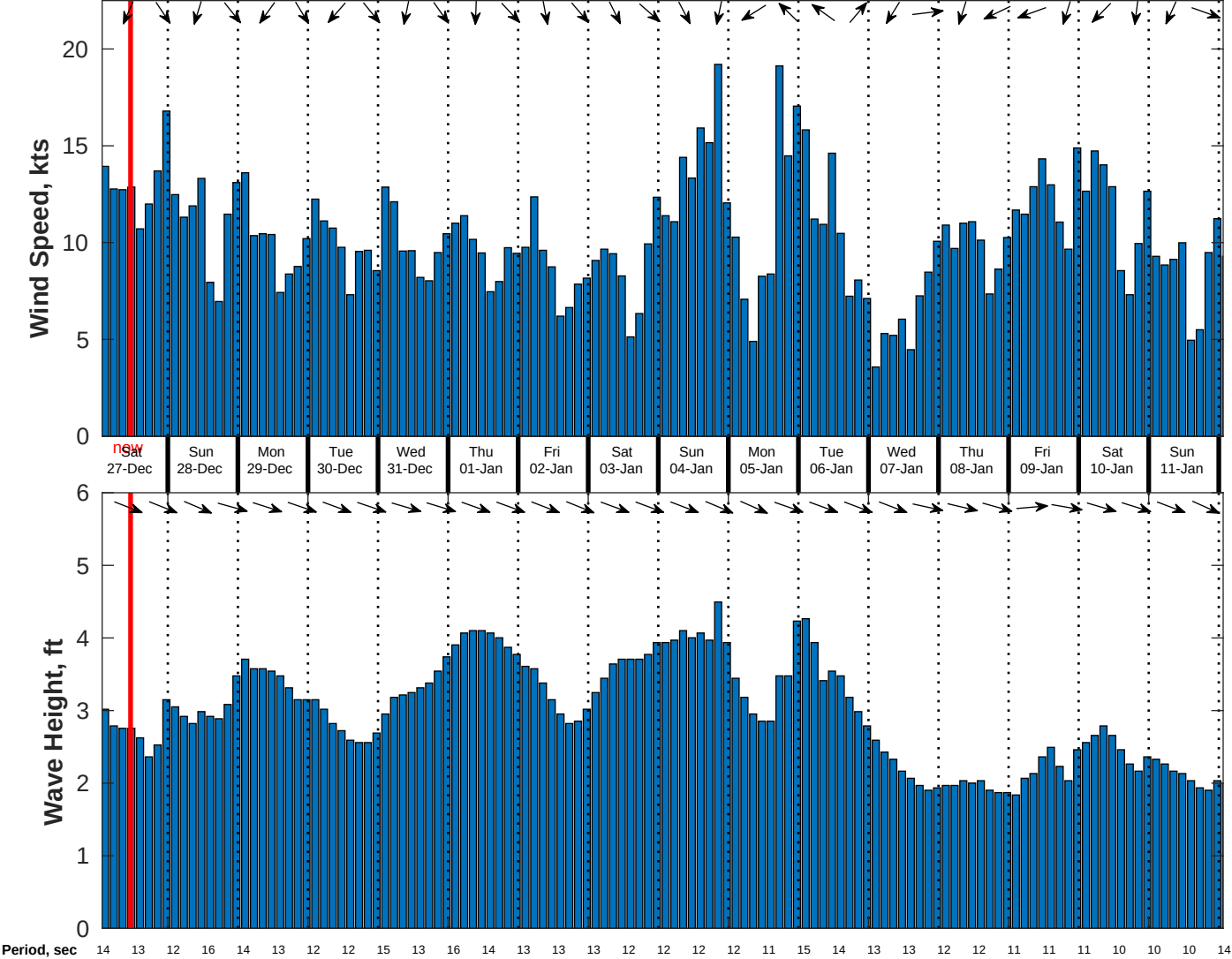
Wind & Wave Forecast for CSA (ONHYM) PPL EBS - Mauritania from 26-Dec-2025 01:00:00 to 11-Jan-2026 01:00:00
