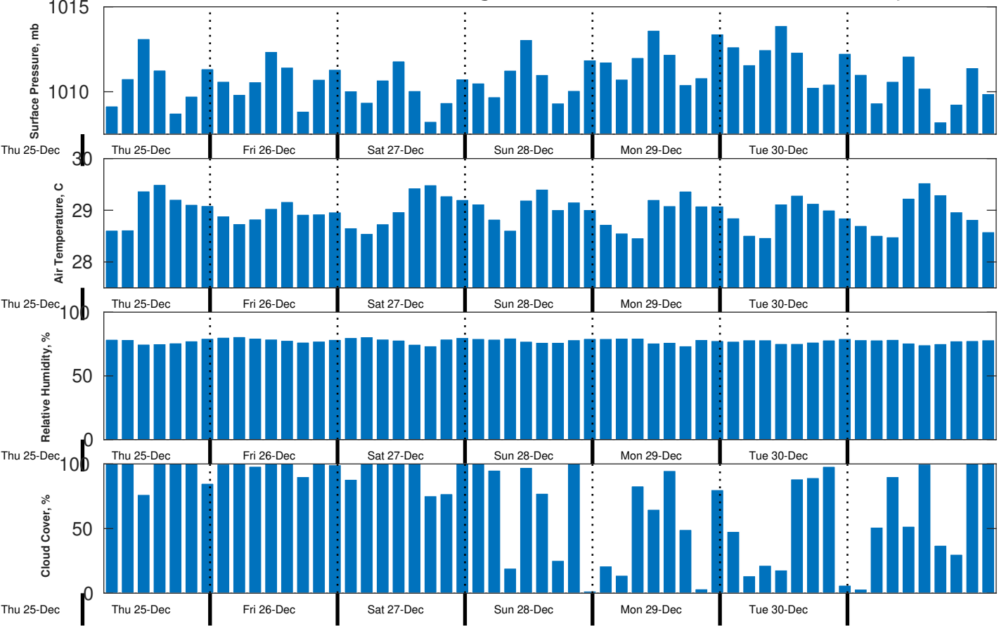
Met Forecast for CSA (ONHYM) PPL EBS - Nigeria from 26-Dec-2025 00:00:00 to 02-Jan-2026 00:00:00
