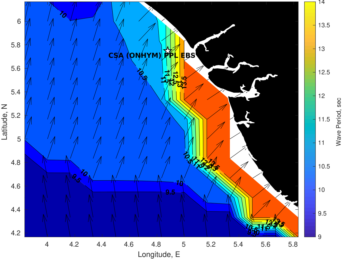
GFS Wave Period (sec) for CSA (ONHYM) PPL EBS - Nigeria at 26-Dec-2025 09:00:00
