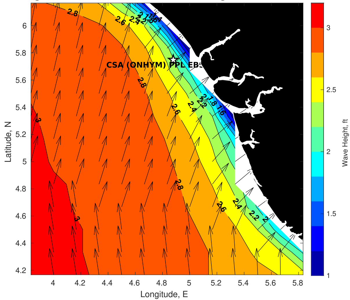
GFS Wave Height (ft) for CSA (ONHYM) PPL EBS - Nigeria at 26-Dec-2025 09:00:00
