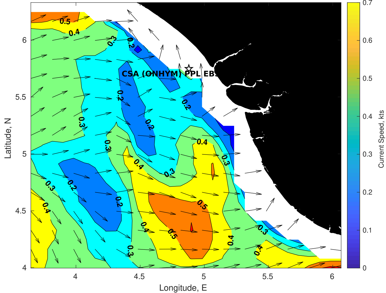
Surface Currents for CSA (ONHYM) PPL EBS - Nigeria at 25-Dec-2025 00:00:00
