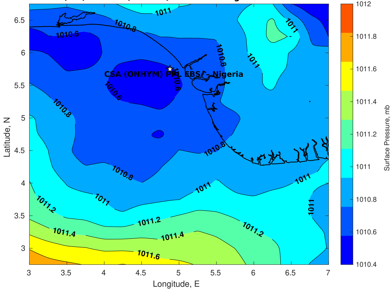
Surface Pressure (mb) for CSA (ONHYM) PPL EBS - Nigeria at 27-Dec-2025 00:00:00
