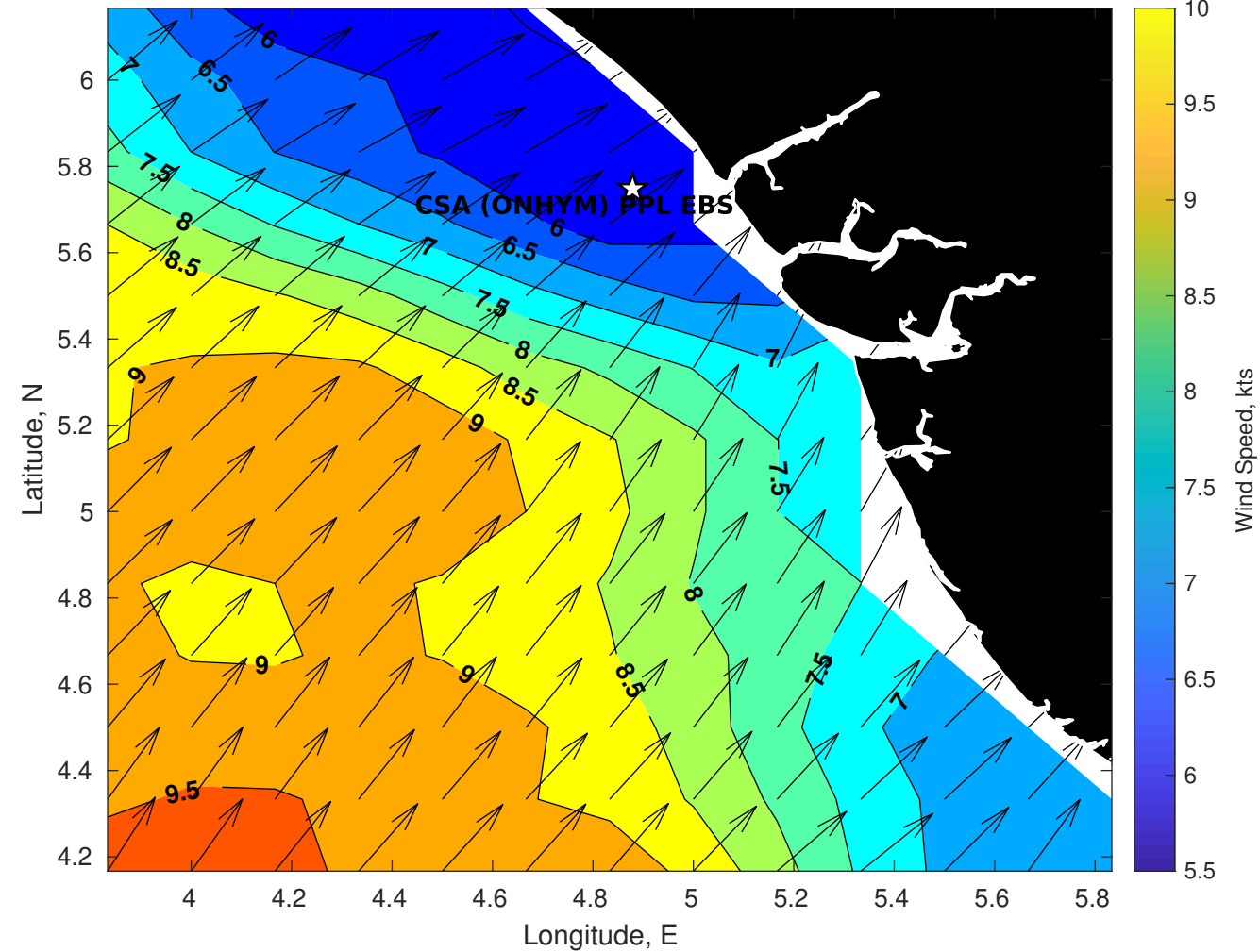
GFS Winds (kts) for CSA (ONHYM) PPL EBS - Nigeria at 26-Dec-2025 09:00:00
