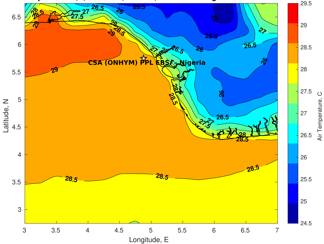
Air Temperature (C) for CSA (ONHYM) PPL EBS - Nigeria at 26-Dec-2025
