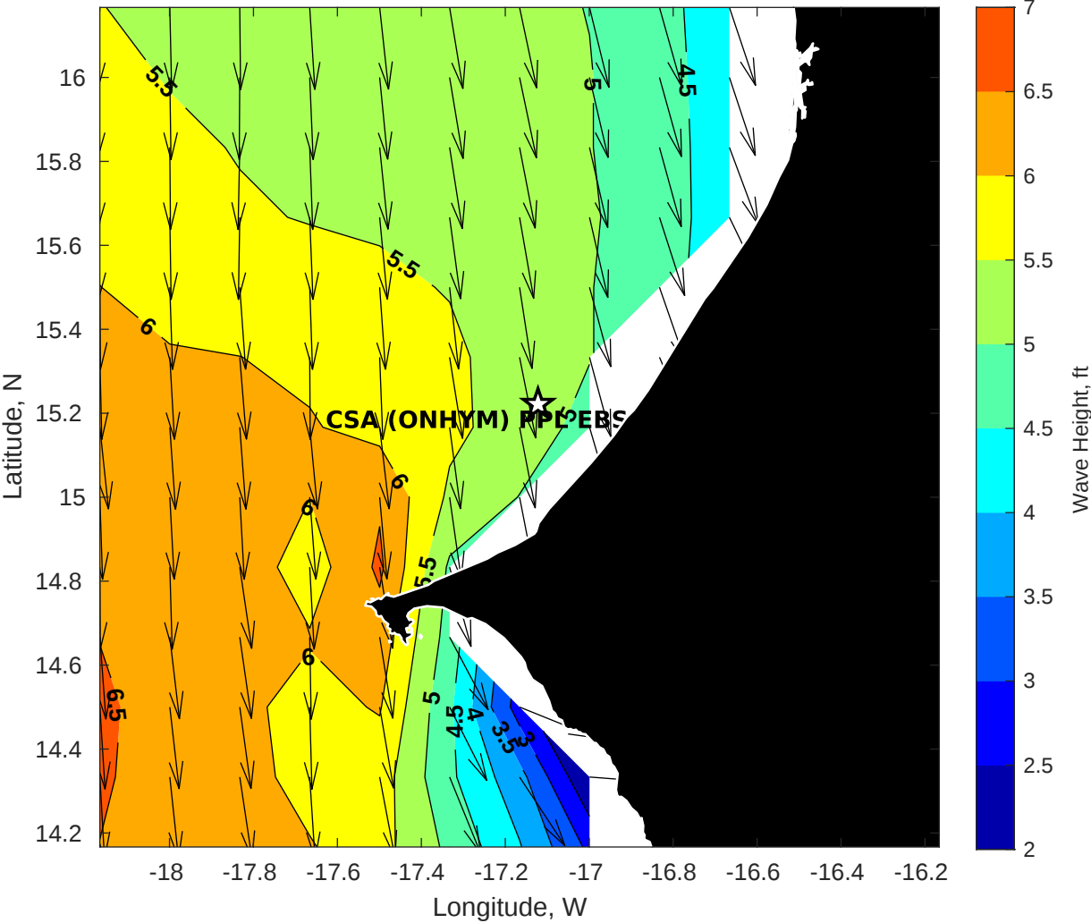
GFS Wave Height (ft) for CSA (ONHYM) PPL EBS - Senegal at 26-Dec-2025 09:00:00
