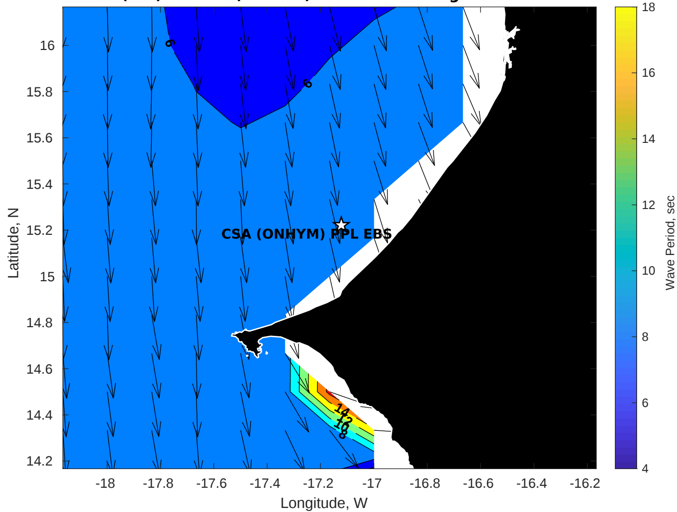
GFS Wave Period (sec) for CSA (ONHYM) PPL EBS - Senegal at 26-Dec-2025 09:00:00
