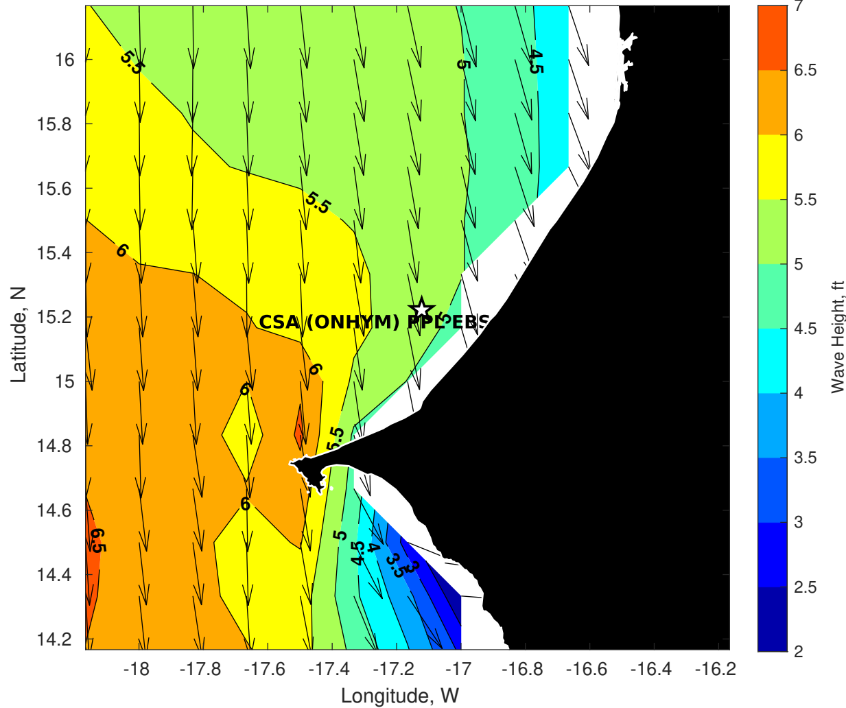
GFS Wave Height (ft) for CSA (ONHYM) PPL EBS - Senegal at 26-Dec-2025 09:00:00
