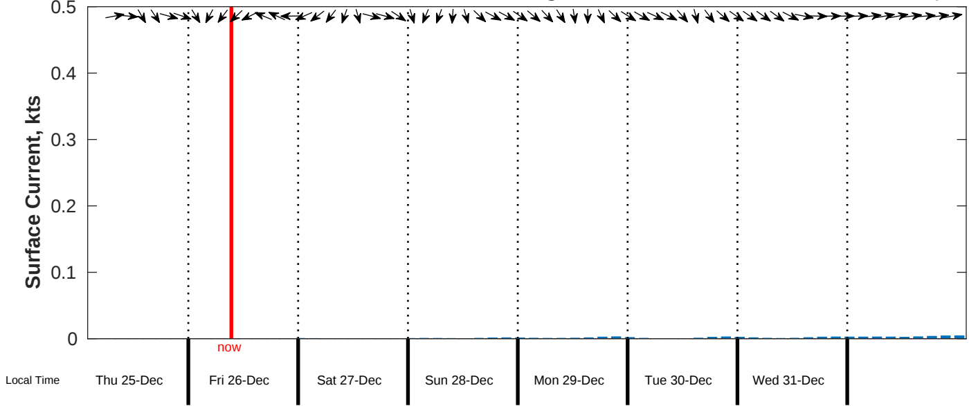
Surface Current Forecast for CSA (ONHYM) PPL EBS - Senegal from 25-Dec-2025 00:00:00 to 02-Jan-2026 00:00:00
