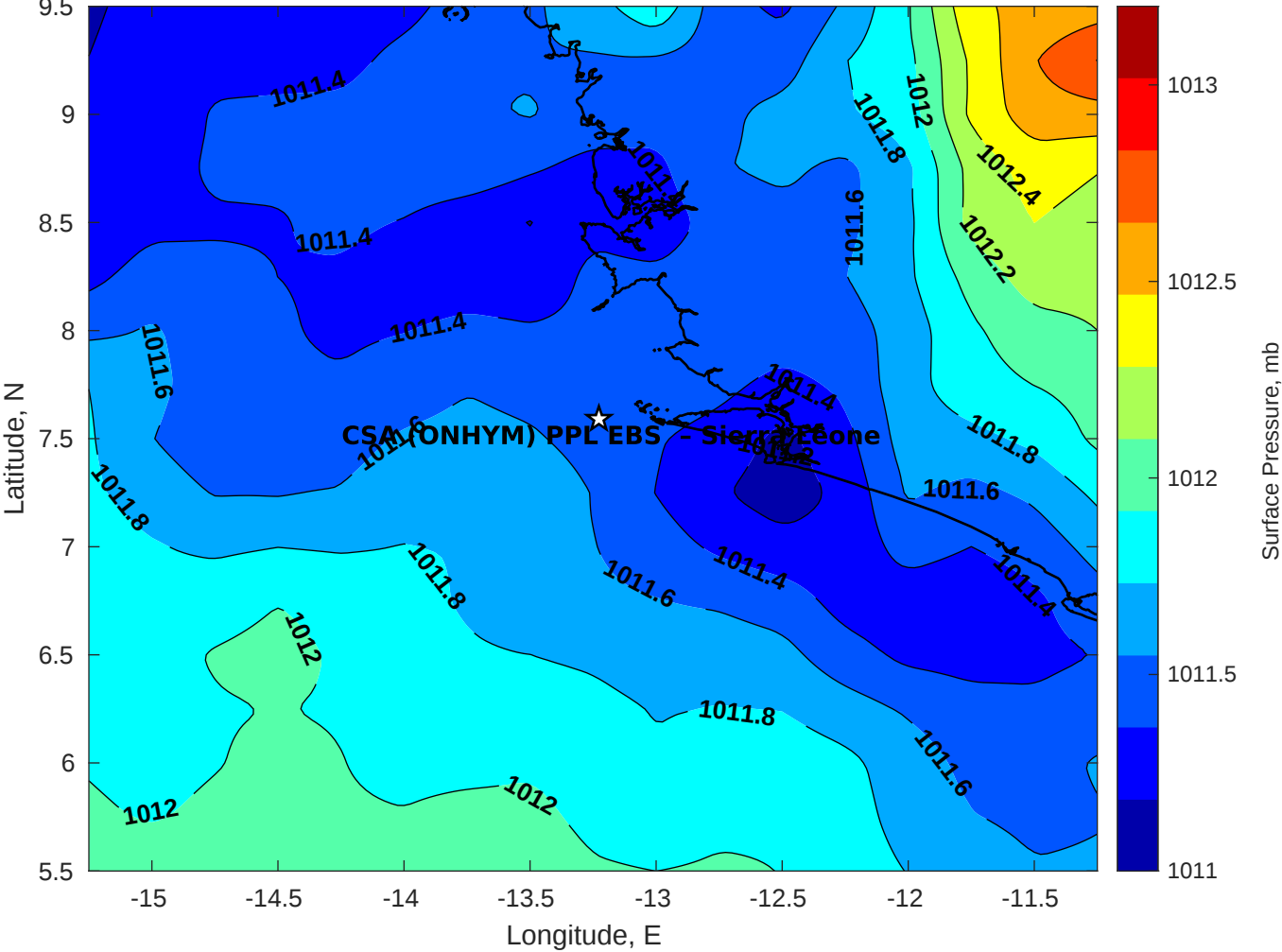
Surface Pressure (mb) for CSA (ONHYM) PPL EBS - Sierra Leone at 26-Dec-2025 00:00:00
