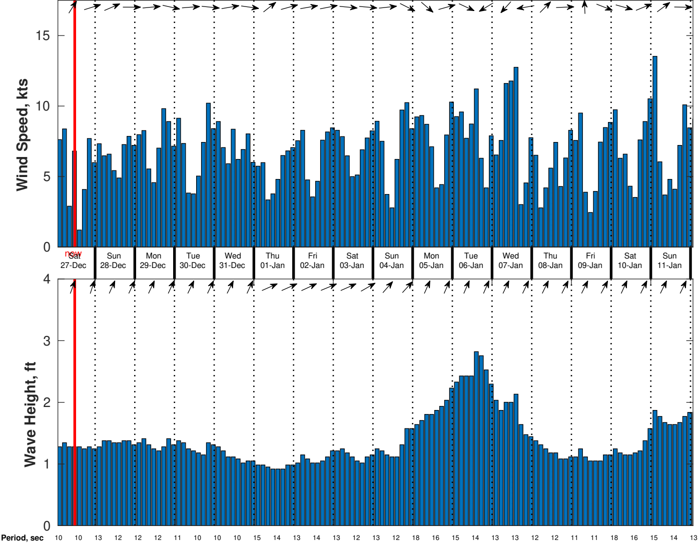
Wind & Wave Forecast for CSA (ONHYM) PPL EBS - Sierra Leone from 26-Dec-2025 01:00:00 to 11-Jan-2026 01:00:00
