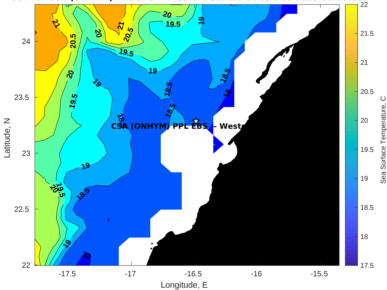
SST for CSA (ONHYM) PPL EBS - Western Sahara at 25-Dec-2025 00:00:00
