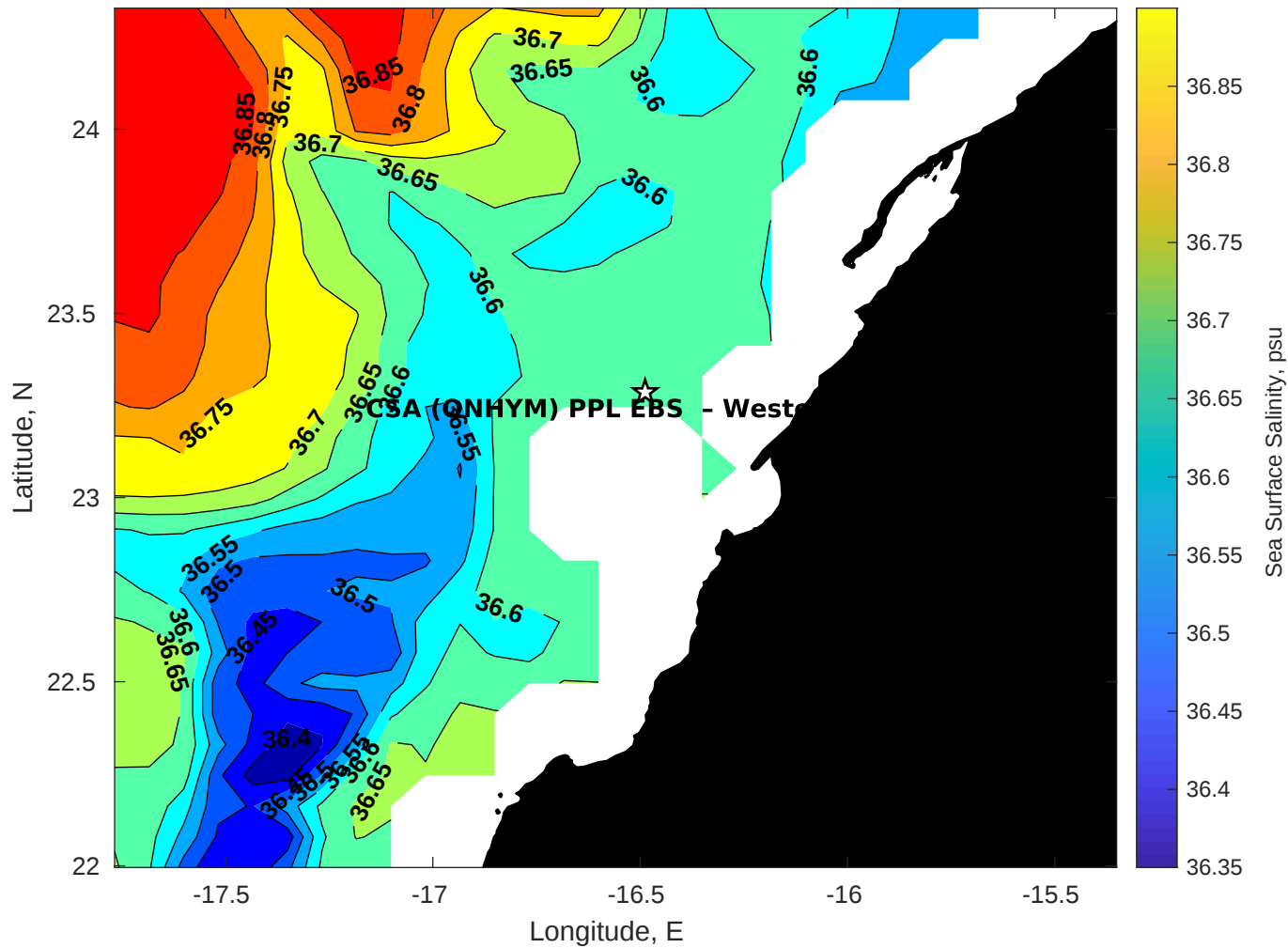
Surface Salinity for CSA (ONHYM) PPL EBS - Western Sahara at 25-Dec-2025 00:00:00
