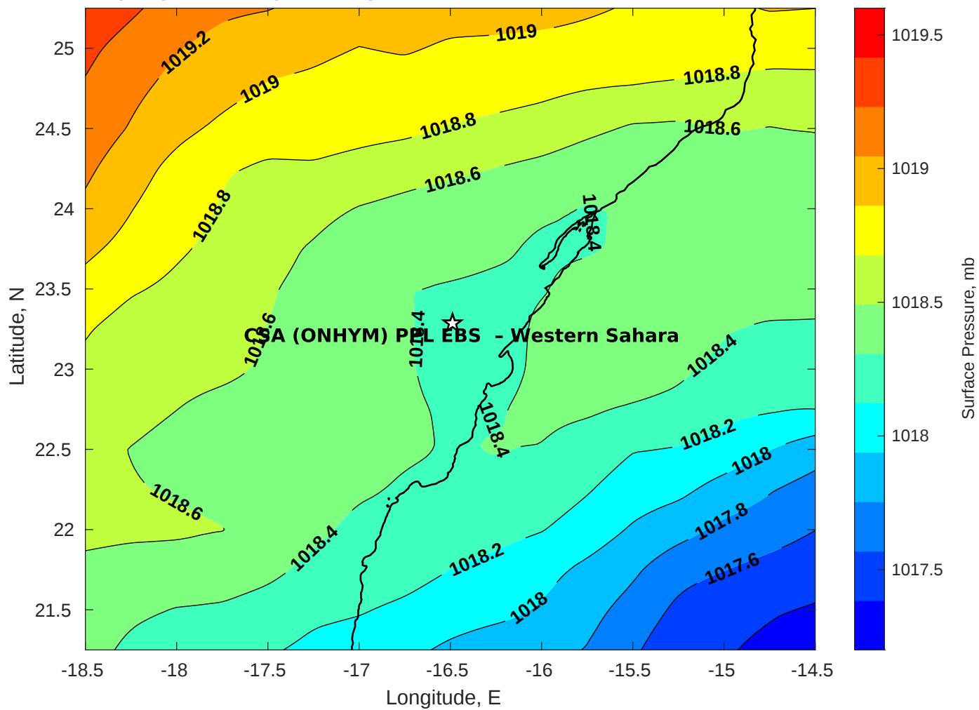
Surface Pressure (mb) for CSA (ONHYM) PPL EBS - Western Sahara at 26-Dec-2025 00:00:00
