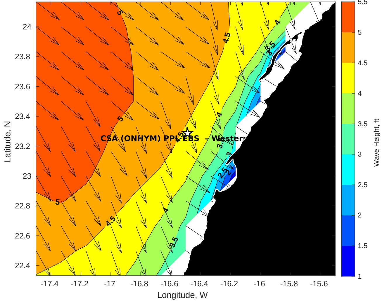
GFS Wave Height (ft) for CSA (ONHYM) PPL EBS - Western Sahara at 26-Dec-2025 09:00:00
