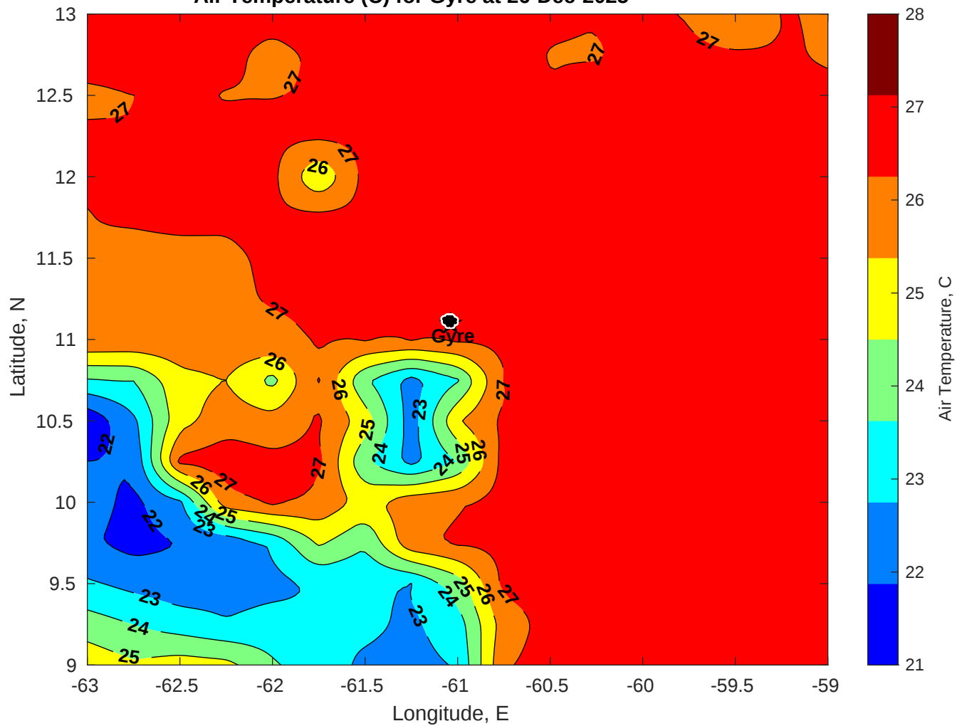
Air Temperature (C) for Gyre at 26-Dec-2025
