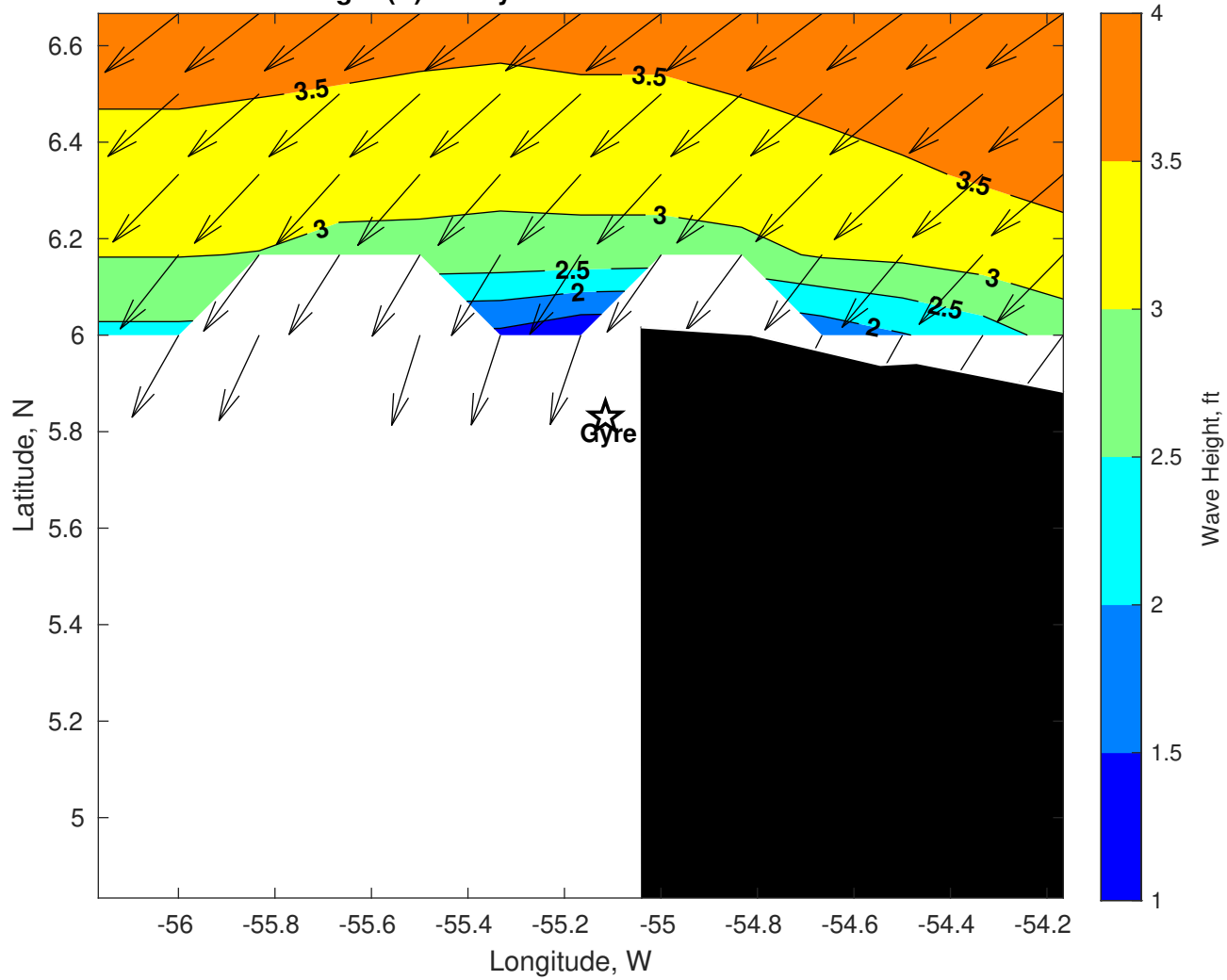
GFS Wave Height (ft) for Gyre at 25-Dec-2025 09:00:00
