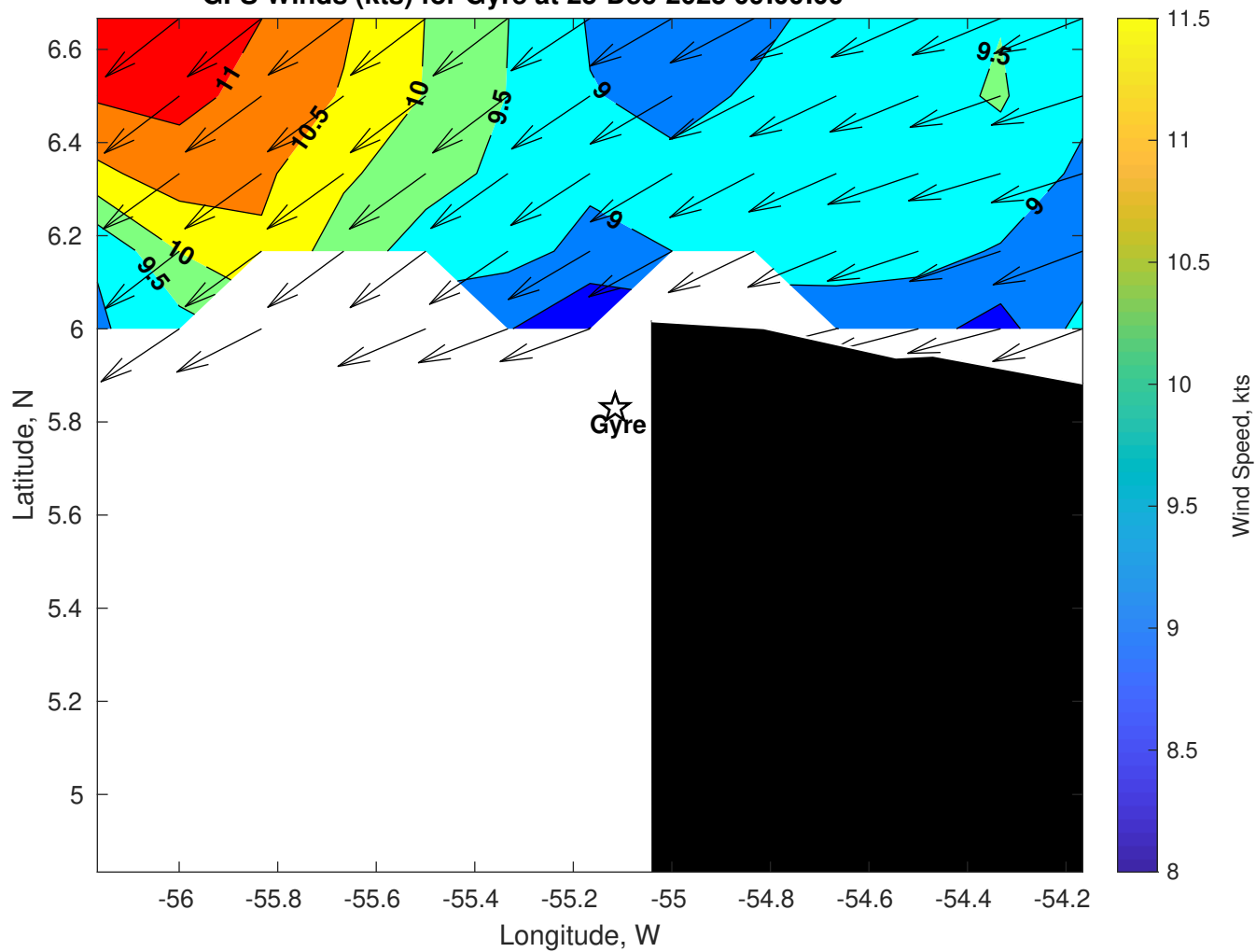
GFS Winds (kts) for Gyre at 25-Dec-2025 09:00:00
