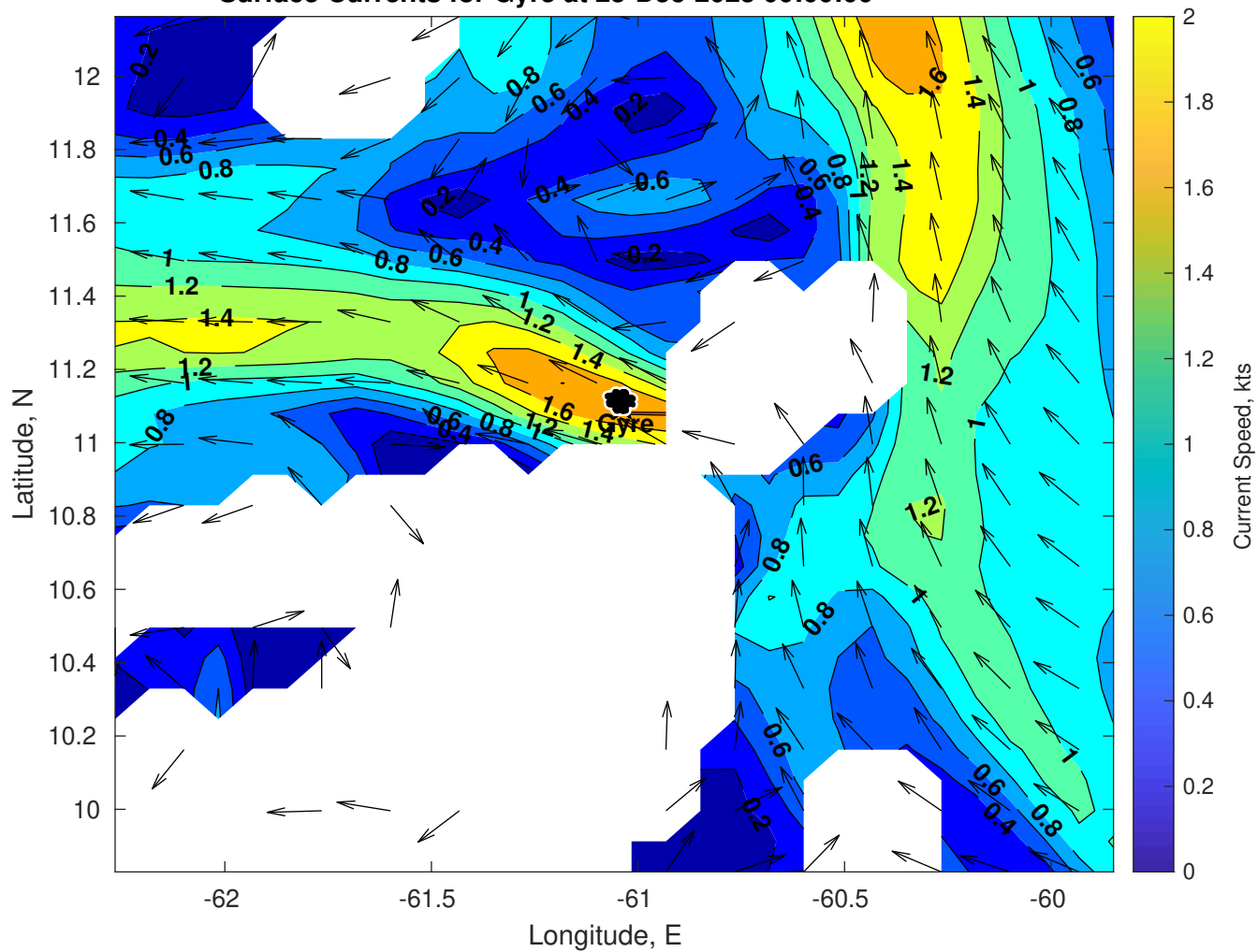
Surface Currents for Gyre at 25-Dec-2025 00:00:00
