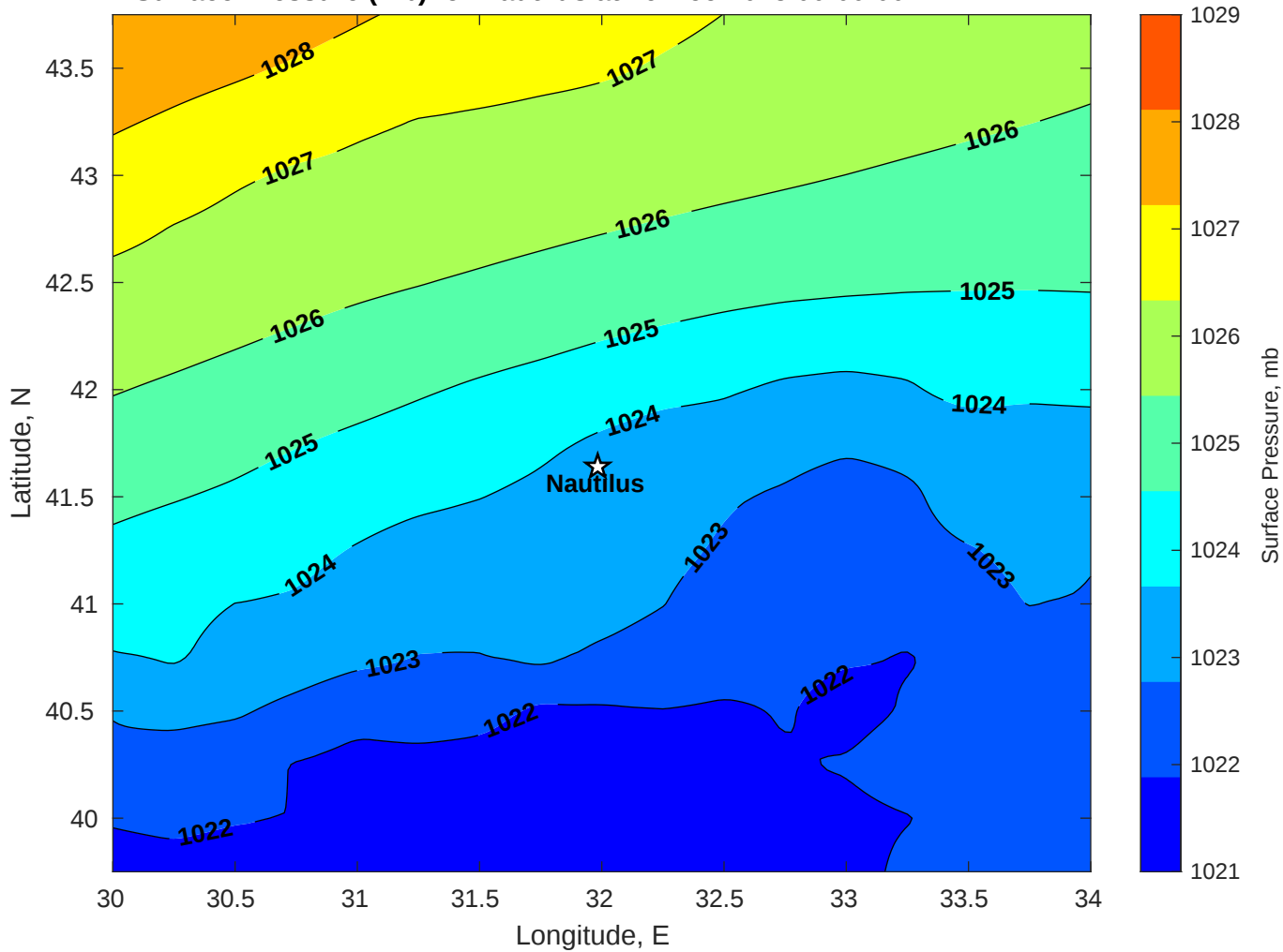
Surface Pressure (mb) for Nautilus at 26-Dec-2025 00:00:00
