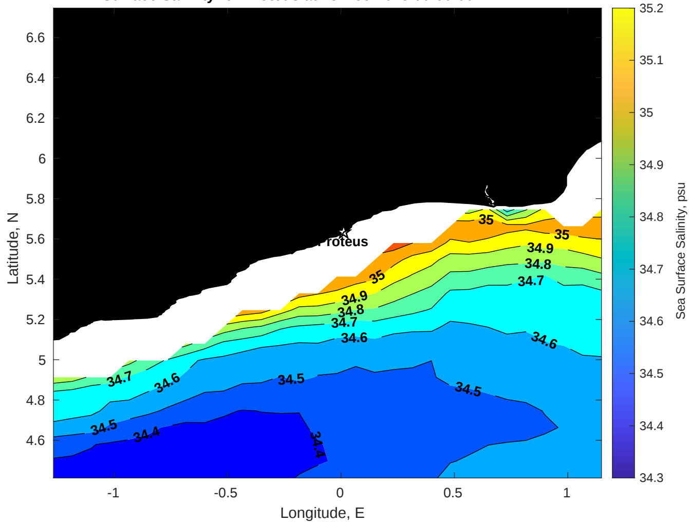
Surface Salinity for Proteus at 25-Dec-2025 00:00:00
