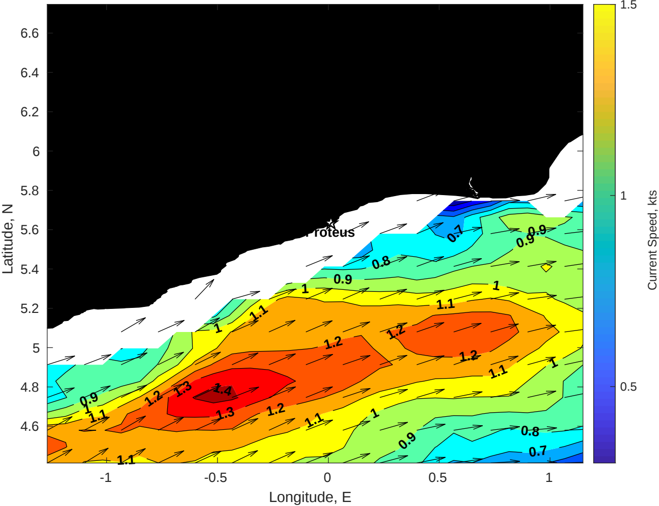
Surface Currents for Proteus at 25-Dec-2025 00:00:00
