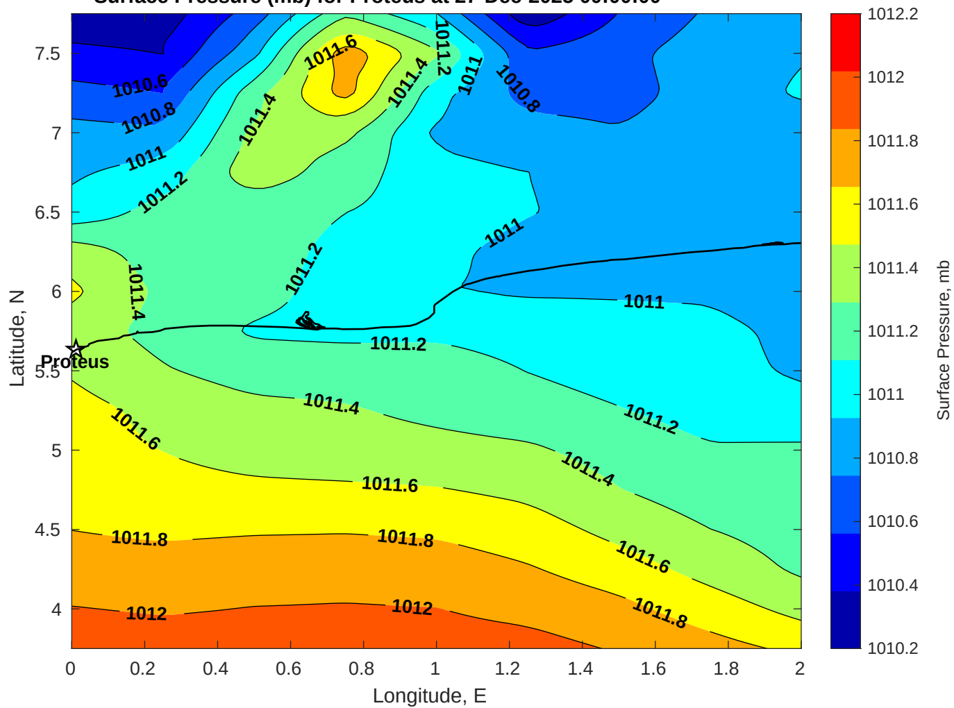
Surface Pressure (mb) for Proteus at 27-Dec-2025 00:00:00
