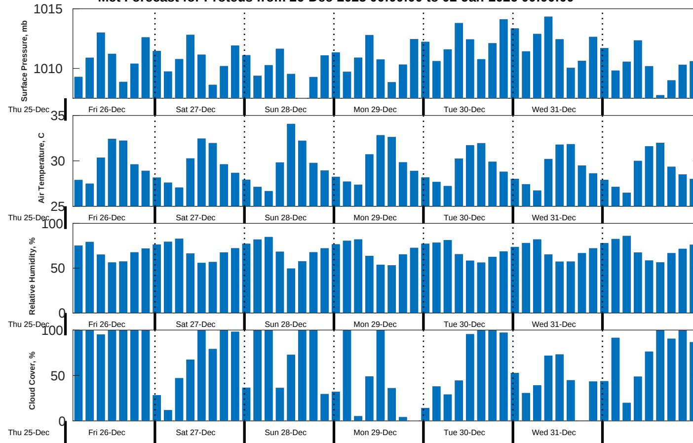
Met Forecast for Proteus from 26-Dec-2025 00:00:00 to 02-Jan-2026 00:00:00
