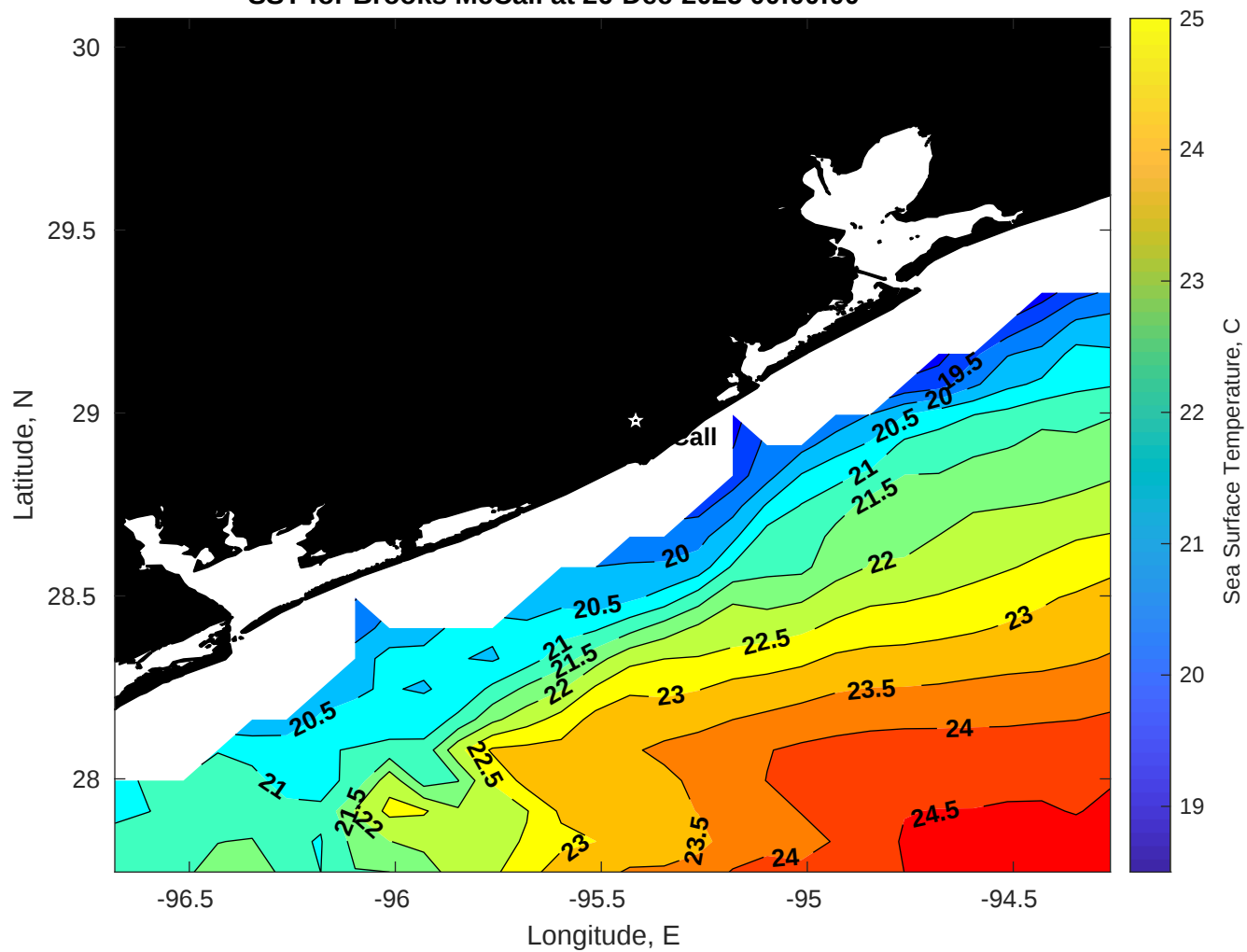
SST for Brooks McCall at 26-Dec-2025 00:00:00
