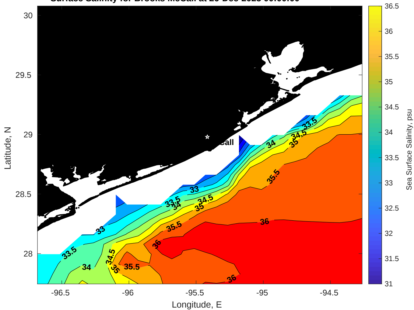
Surface Salinity for Brooks McCall at 26-Dec-2025 00:00:00
