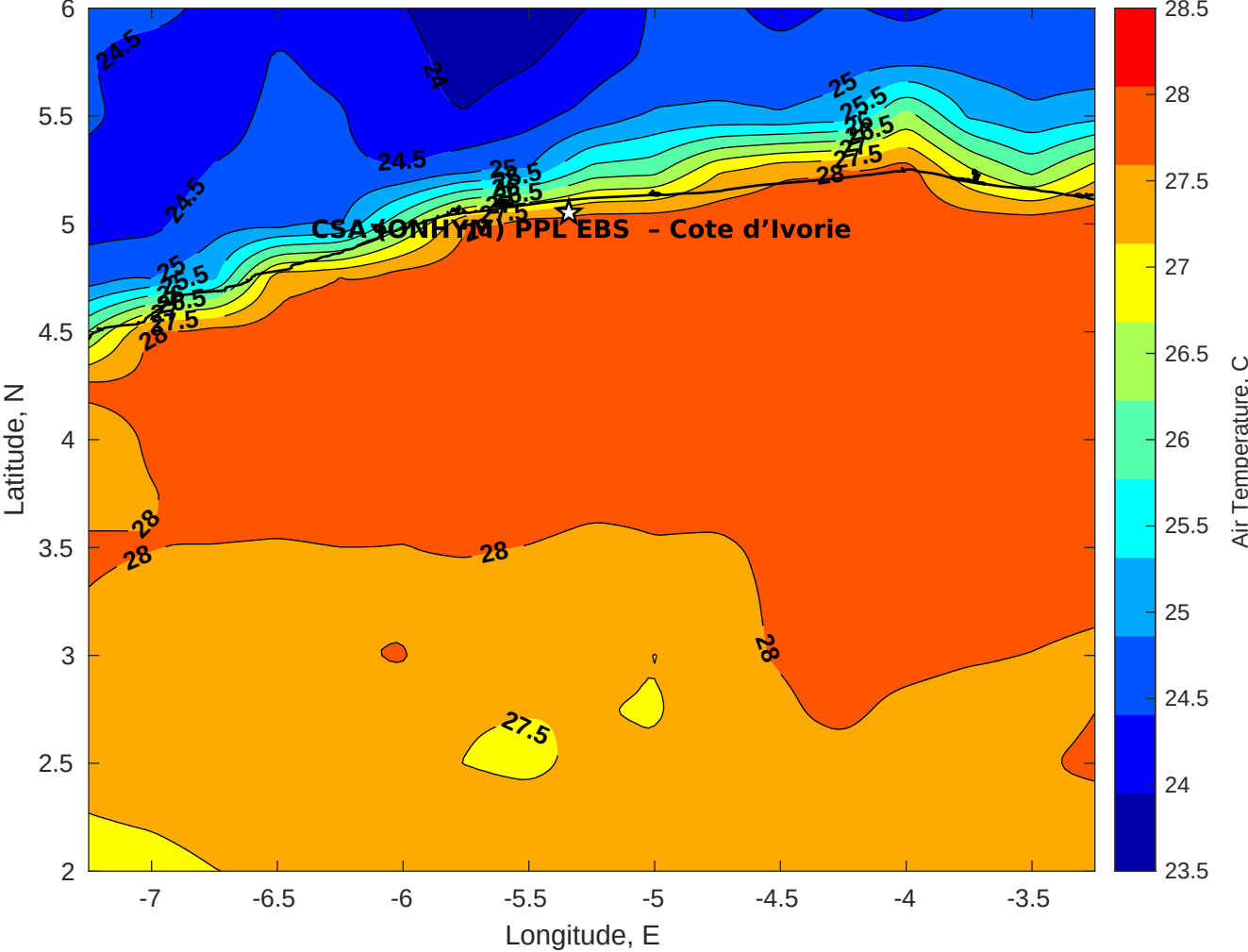
Air Temperature (C) for CSA (ONHYM) PPL EBS - Cote d'Ivoire at 27-Dec-2025
