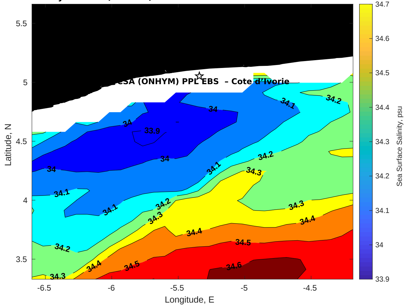
Surface Salinity for CSA (ONHYM) PPL EBS - Cote d'Ivoire at 26-Dec-2025 00:00:00
