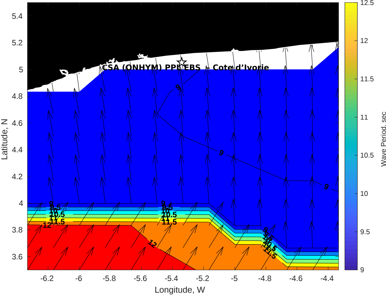
GFS Wave Period (sec) for CSA (ONHYM) PPL EBS - Cote d'Ivoire at 27-Dec-2025 09:00:00
