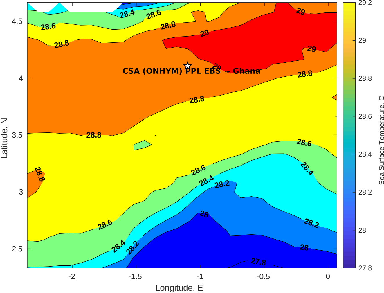
SST for CSA (ONHYM) PPL EBS - Ghana at 26-Dec-2025 00:00:00
