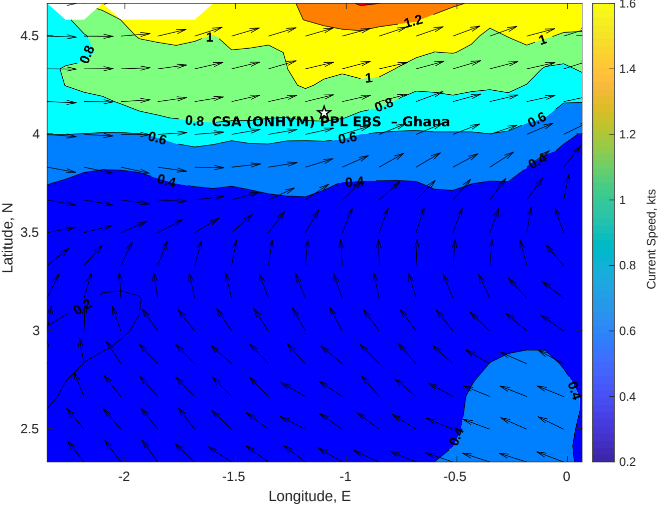
Surface Currents for CSA (ONHYM) PPL EBS - Ghana at 26-Dec-2025 00:00:00
